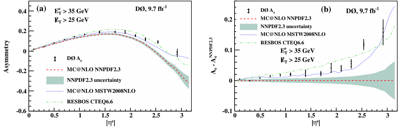
FIG. 17 (color online). The electron charge asymmetry distribution after CP folding with asymmetric kinematic cuts E_T^e > 35 GeV, E_T > 25 GeV. (a) Comparison between the measured asymmetry and predictions and (b) the differences between the data and MC predictions and the predicted central value from MC@NLO using the NNPDF2.3 PDF set. The black dots show the measured electron charge asymmetry, with the horizontal bars showing statistical uncertainty and the vertical lines showing the total uncertainty. The red dashed lines and cyan bands are the central value and uncertainty band from MC@NLO, respectively, using the NNPDF2.3 PDF sets. The blue dotted lines show the prediction from MC@NLO using the MSTW2008NLO central PDF set, and the green dot-dashed lines show the prediction from RESBOS using the CTEQ6.6 central PDF set.
