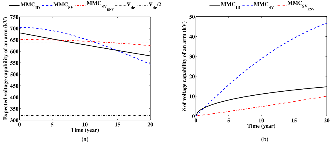
Fig. 10. (a) Expected voltage capability of an arm and (b) the corresponding standard deviation—Design to meet Reliability \geq 0.998 in the first three years.
