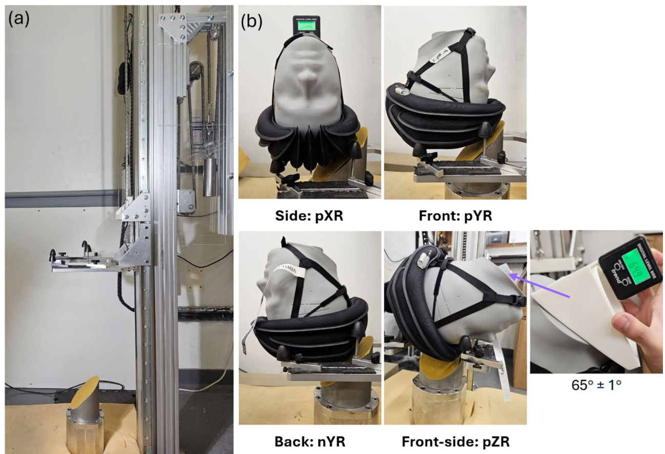
Fig. 2. (a) The drop tower test rig. (b) The four tested impact locations. Here X, Y and Z refer to the axis of the dominant rotational velocity component and R refers to rotation. The direction of rotation is indicated by p (positive) and n (negative).
