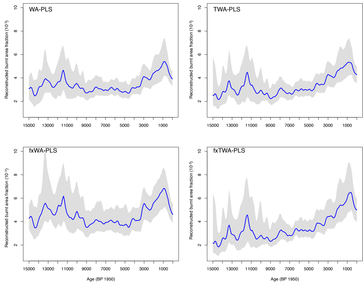
175 Figure S6. Composite curves of reconstructed burnt area using WA-PLS and TWA-PLS, with and without fx correction, using the locfit() function with half-width = 300, number of bootstrap samples = 1000. The locally estimated scatterplot smoothing is shown in blue; The upper and lower 95th-percentile confidence intervals are shown in grey.
