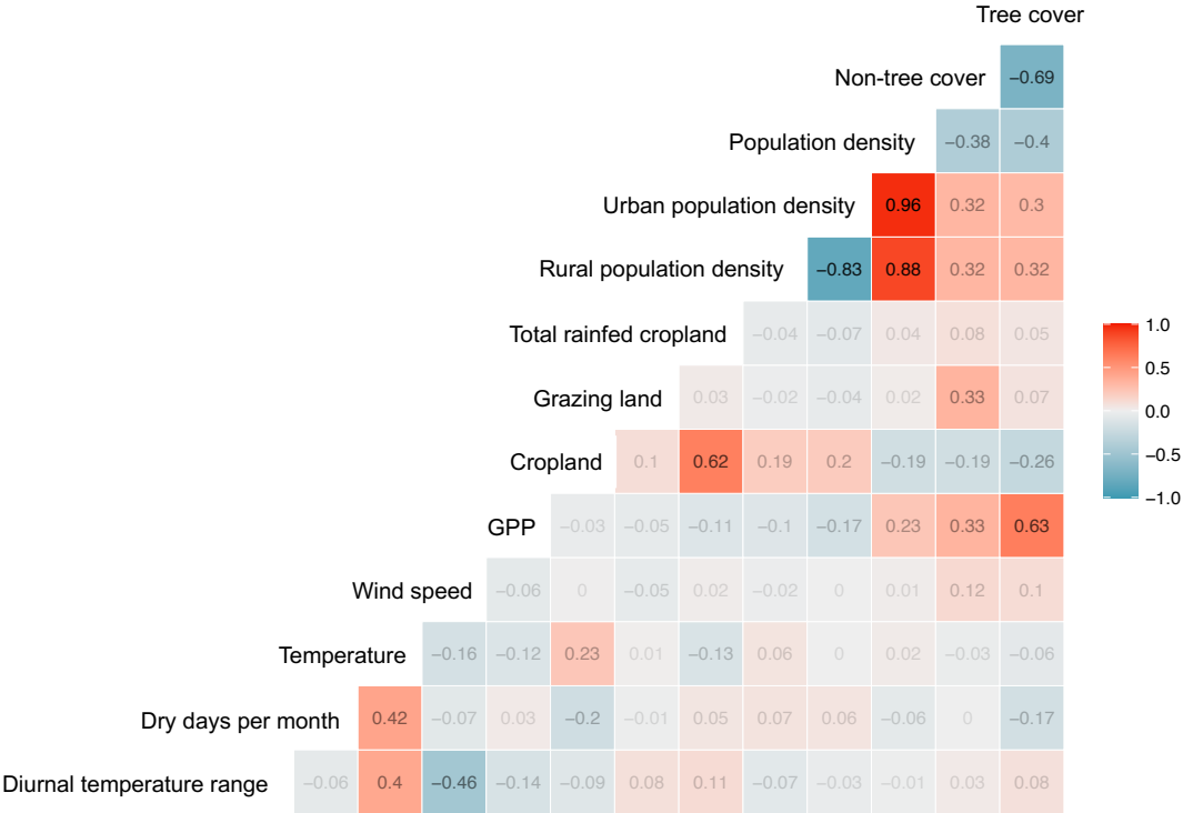
105 Figure S1. Partial correlations test based on data sets for the Iberian Peninsula that include annual observations at 0.5° for the period between 2001 and 2016. The data are all transformed according to Table S5 prior to the test.
