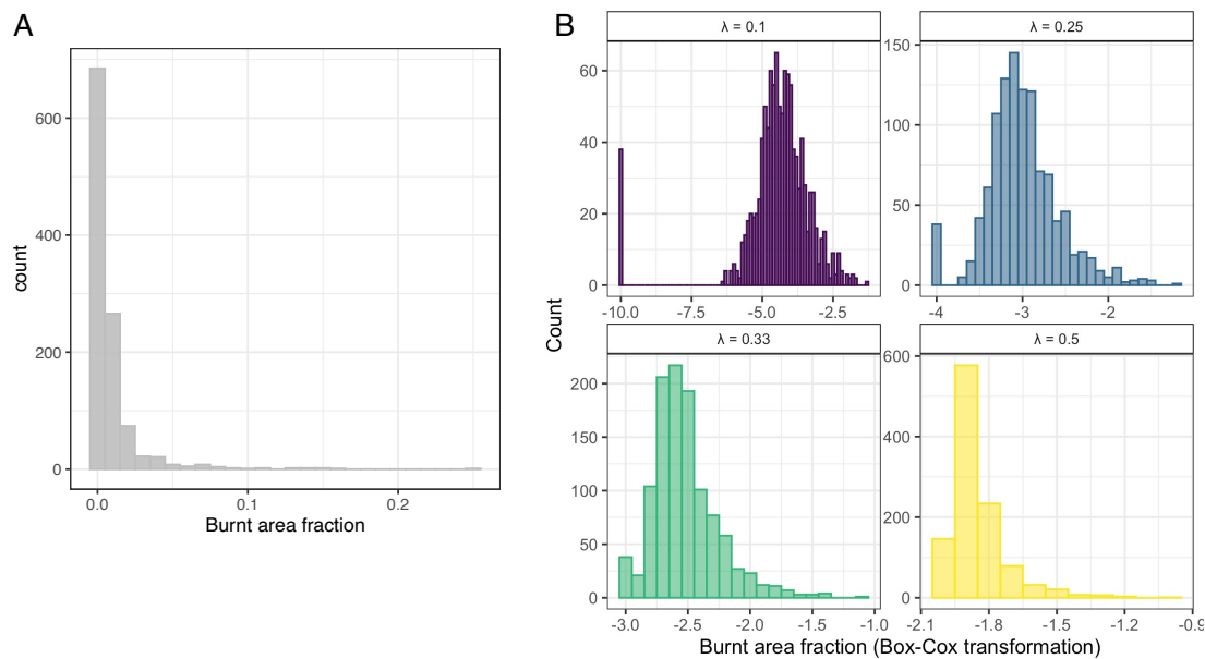
Figure S3. Distribution of palaeo burnt area fraction before (Panel A) and after (Panel B) Box-Cox transformation.
