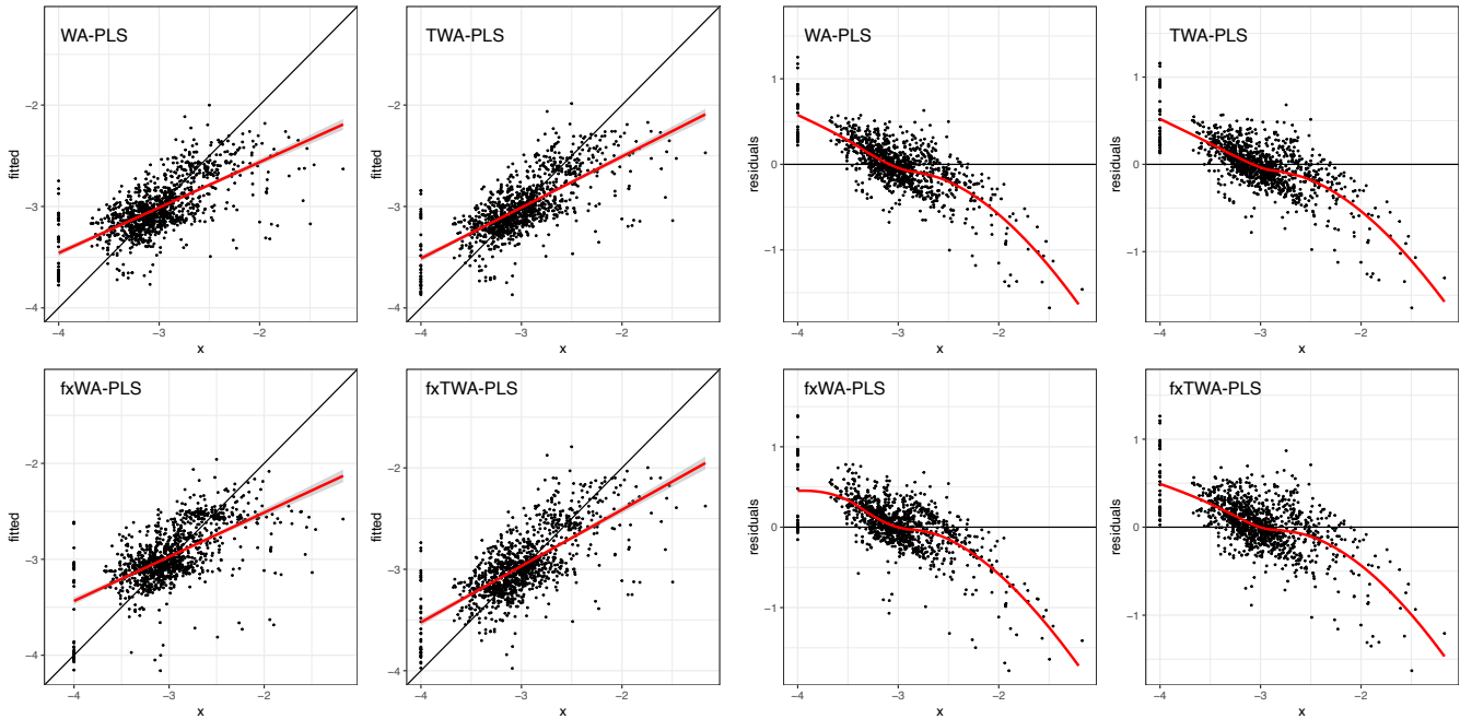
Figure S5. The fitted plots and residual plots of WA-PLS and TWA-PLS methods, with and without fx correction.
