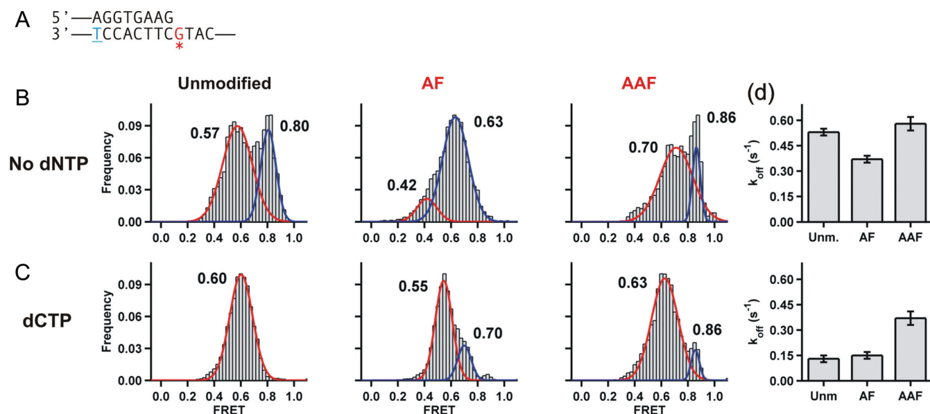
Figure 2. Carcinogenic adducts at the templating base distort polymerase binding to DNA. (A) Primer-template sequence used to study Dpo4 binding. A complete sequence is shown in Supplementary Table S1. The blue underlined T in the template is conjugated to a Cy3 dye, while the red starred G marks the position of the carcinogen adducts. (B) FRET efficiency histograms for Dpo4 binding to unmodified, AF-modified and AAF-modified primer-templates in the absence of nucleotide. All FRET distributions were fit with two Gaussian functions shown as red and blue lines. (C) FRET histograms for Dpo4 binding the same DNA constructs as (B) in the presence of the next correct nucleotide dCTP. (D) Dpo4 dissociation rates from unmodified, AF-modified and AAF-modified primer-templates for the binary (top) and ternary complexes (bottom).
