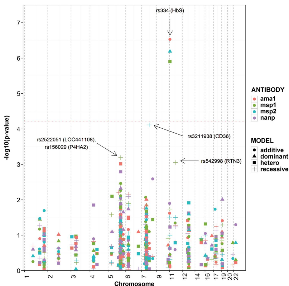
Fig. 4 Plot for 178 SNPs with logged anti-malarial antibody levels. Values of -\log_{10} p-values plotted against chromosomal positions; only the lowest meta-analysis p-value for each SNP-antibody association is plotted. The red dotted line indicates a Bonferroni threshold p-value of 6 \times 10^{-5} . Each colour represents a different anti-malarial antibody while the shape of the point represents the genetic model of best fit for the SNP-antibody association: (circle) for additive, (triangle) for dominant, and (square) for heterozygote and (plus) for recessive. Adjusted for age, gender, microscopy result, village (>20), ethnicity (>20), sample month (>20) and study.
