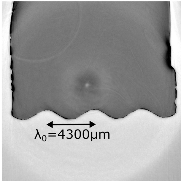
FIG. 3. A single 2D slice of a 3D synchrotron-tomography of an aerogel sample ( \lambda_0 = 4300 \mu\text{m} , a_0/\lambda_0 \sim 0.2 ) obtained prior to an experiment. Bright regions correspond to low x-ray attenuation (low density), while darker regions correspond to higher densities. The air-aerogel interface is highlighted via x-ray phase contrast imaging and shows high-frequency low-amplitude perturbations characteristic of all manufactured samples.
