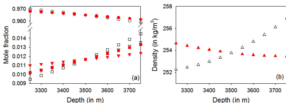
Fig. 1 Simulated species distribution a and density b of a condensate gas (cell E) as a function of depth. Open black symbol: only gravitational segregation. Solid red symbols: thermogravimetric diffusion included in the model. Left panel a : C1 (circles), nC7 (triangles) and nC10 (squares)
