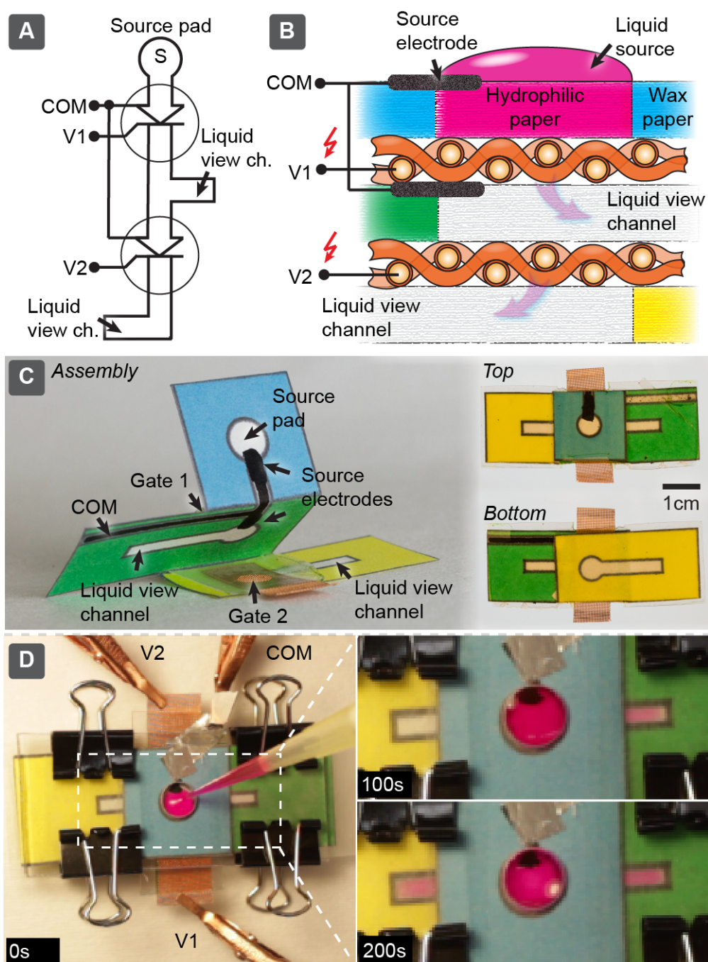
Figure 4. Valves in serial connection. (A) Circuit diagram of two individually addressable electrofluidic valves connected in series. We have used liquid view channels to visualize the
