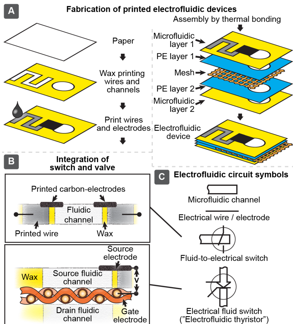
Figure 2. Design and fabrication of printed electrofluidic devices. (A) Schematic diagram of the fabrication of three-dimensional printed electrofluidic circuits. Microfluidic channels are printed using wax printing, followed by printing of electrodes (for valves and switches) and electrical wires on the paper layers. Conductive, insulated, and hydrophobic "electrotextiles" are then bonded with the paper layers using hot-lamination with polyethylene films. (B) Schematic cross-section of a fluid-to-electrical switch, and Schematic cross-section of an integrated valve, containing two microfluidic layers, and a valve layer. The valve is actuated when a voltage is applied between the liquid ("source electrode") and the electrotextile ("gate electrode") whereupon liquid can pass from the "liquid source" into the "liquid drain". (C)
