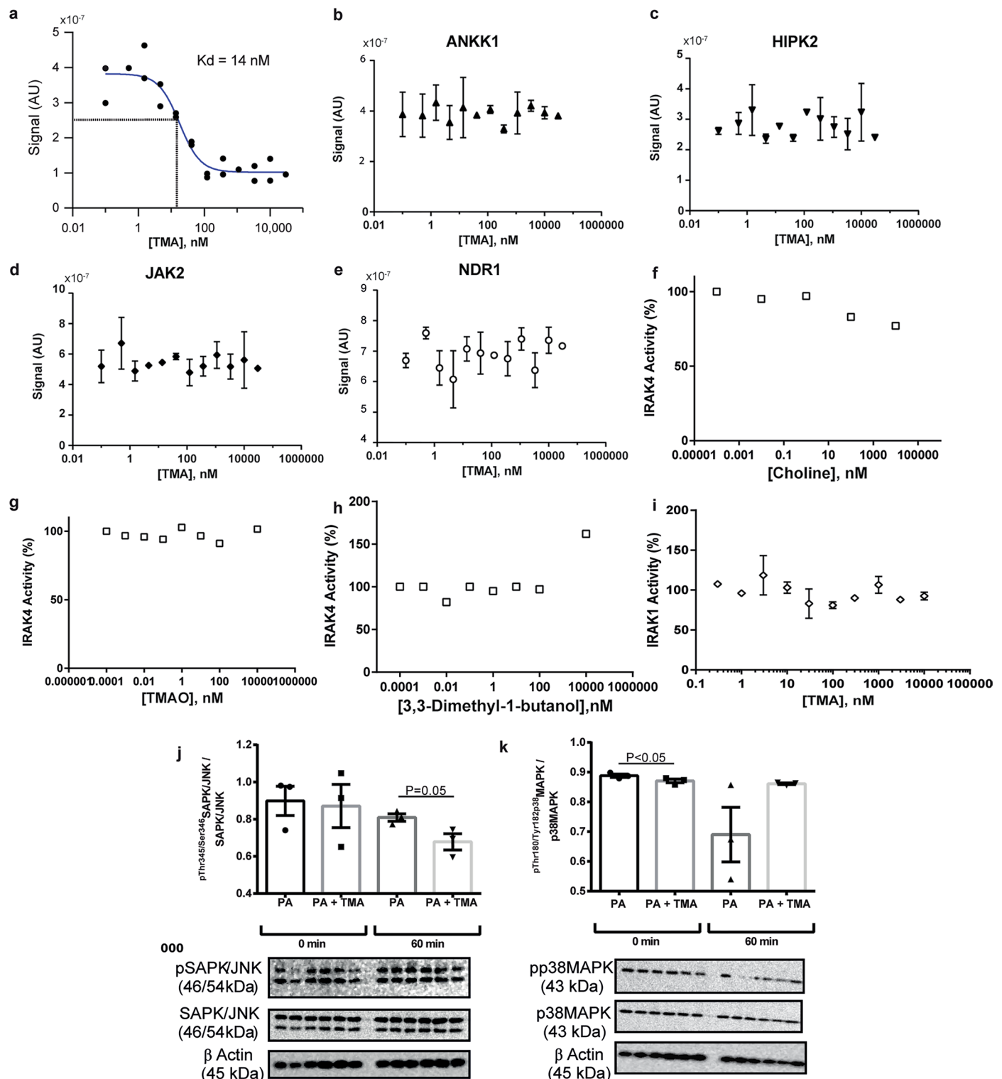
Extended Data Fig. 5 | TMA does not bind with kinases ANKK1, HIPK2, JAK2, and NDR1 identified as candidates in the kinome screen, but makes significant contact with IRAK4. (a) Confirmation of a physical interaction between TMA and IRAK4 using TMA at concentrations ranging from 0.1 nM to 100 \mu\text{M} , resulting in a dissociation constant ( K_d ) of 14 nM. (b–e) Physical interaction test between TMA and the four hits identified using a kinome screen, using TMA concentrations ranging from 0.1 nM to 100 \mu\text{M} for (b) ANKK1, (c) HIPK2, (d) JAK2 and (e) NDR1. For (b–e) N = 2 biological repeats. IRAK4 kinase activity
