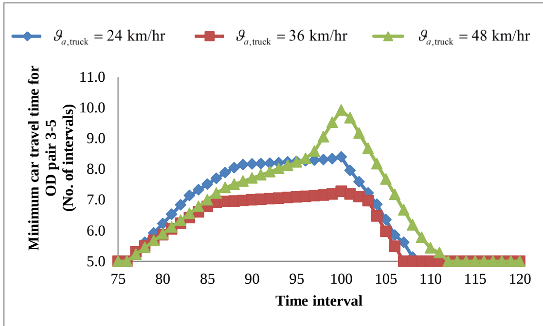
(c) Effect of truck speed on the minimum car travel time for OD pair 3-5
