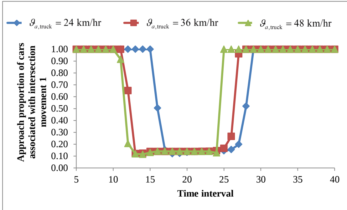
(a) Effect of truck speed on the approach proportions of cars in OD pair 0-5
