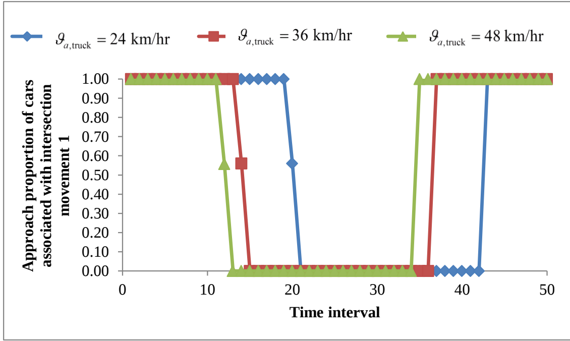
(a) Effect of truck speed on the approach proportions of cars
