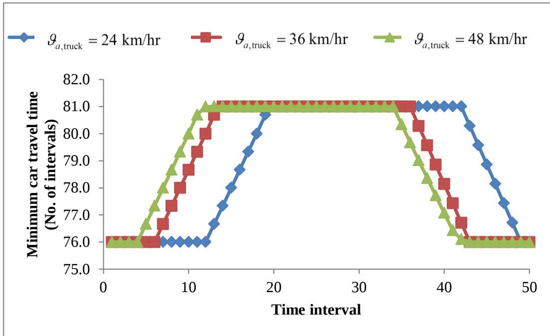
(b) Effect of truck speed on the travel times of cars
