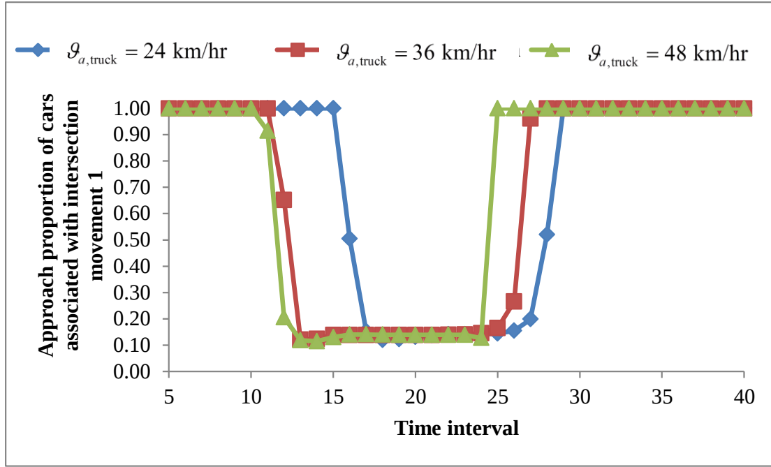
(b) Effect of truck speed on the minimum travel time for OD pair 0-5
