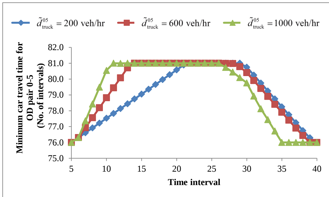
(b) Effect of truck demand on the minimum car travel time for OD pair 0-5
