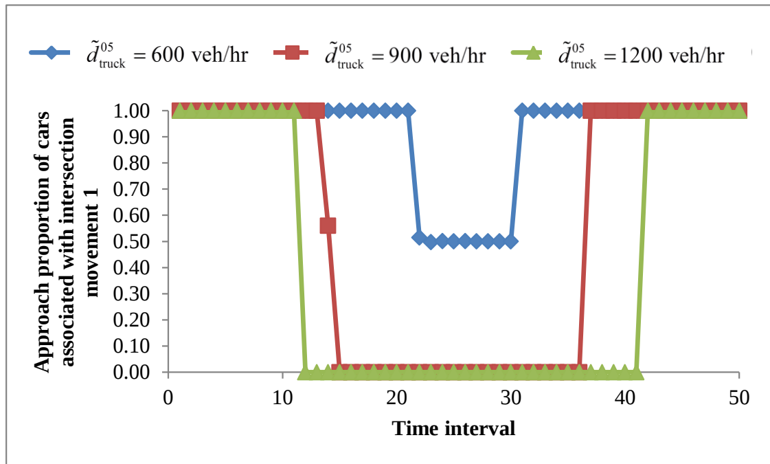
(a) Effect of truck demand on the approach proportions of cars
