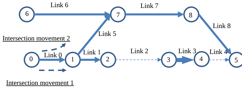
Figure 7 Nine-node small network
