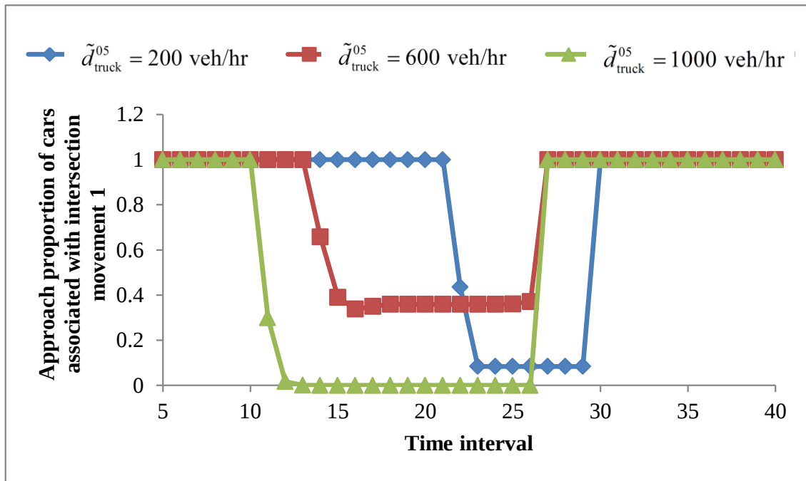
(a) Effect of truck demand on the approach proportions of cars in OD pair 0-5
