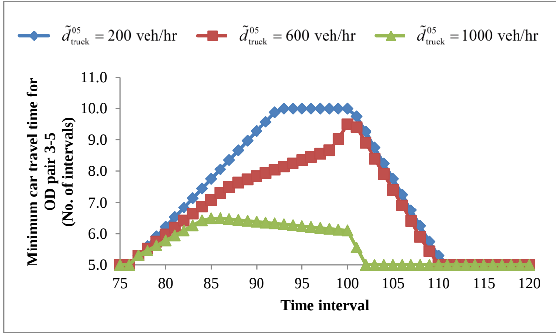
(c) Effect of truck demand on the minimum car travel time for OD pair 3-5
