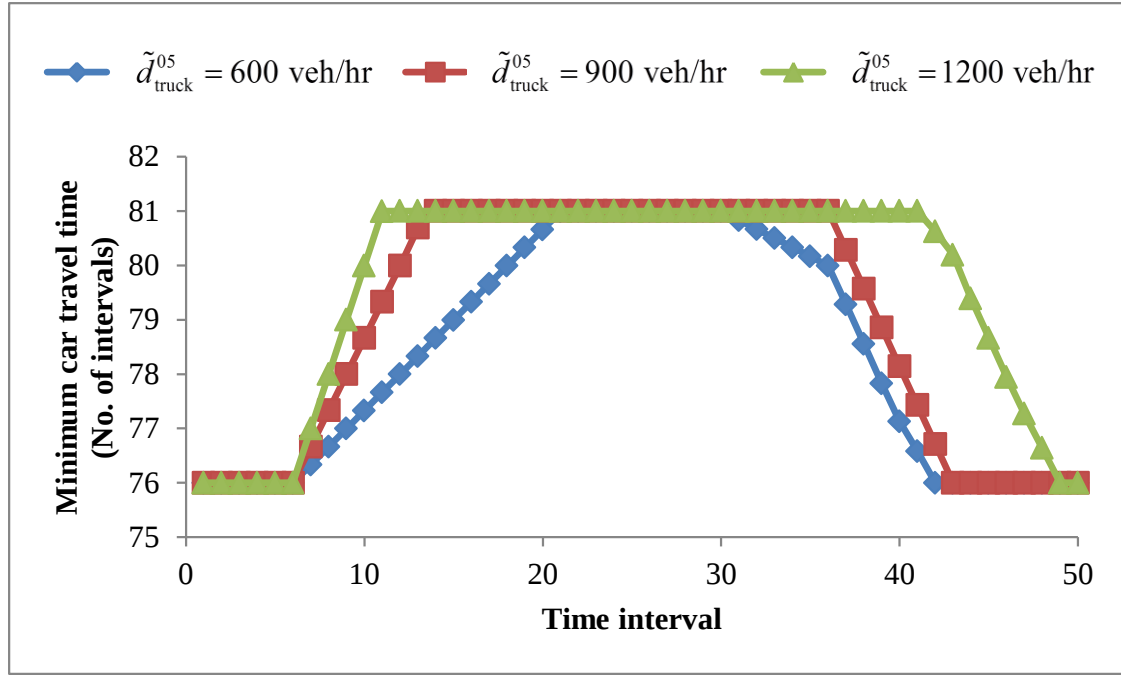
(b) Effect of truck demand on the travel times of cars
