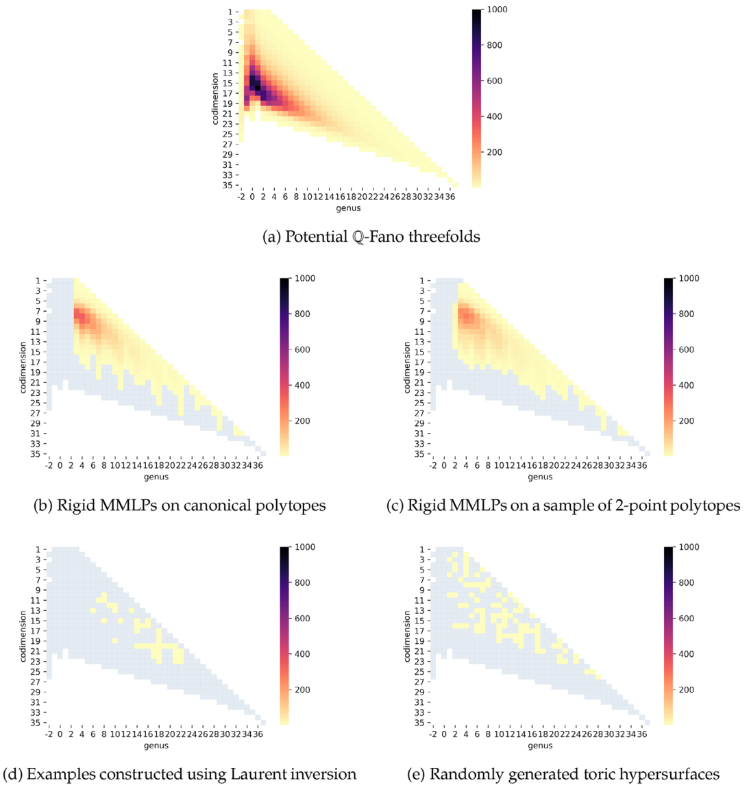
FIGURE 1 The distribution of potential Hilbert series for \mathbb{Q} -Fano threefolds with Fano index 1: (a) from the Graded Ring Database; (b) from mutation-equivalence classes of rigid MMLPs with three-dimensional canonical Newton polytope; (c) from mutation-equivalence classes of rigid MMLPs with Newton polytope in a random sample of three-dimensional polytopes with two interior points; (d) from toric complete intersections constructed using Laurent inversion; (e) from randomly generated quasismooth hypersurfaces in toric orbifolds of Picard rank 2. Hilbert series are recorded as pairs (c, g) where c is the estimated codimension and g = g(X) is the genus. Plots (b)–(e) have the shadow of plot (a) as background.
