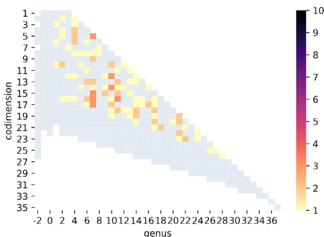
FIGURE 13 The distribution of Hilbert series for randomly generated \mathbb{Q} -Fano quasismooth threefold hypersurfaces in \mathbb{Q} -factorial toric varieties of Picard rank 2. Hilbert series are recorded as pairs (c, g) where c is the estimated codimension and g is the genus.
