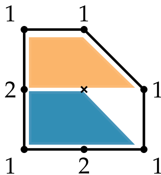
FIGURE 8 A scaffolding of f with shape \mathbb{F}_1 .
