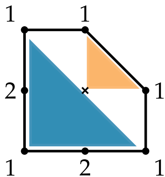
FIGURE 7 A scaffolding of f with shape \mathbb{P}^2 .
