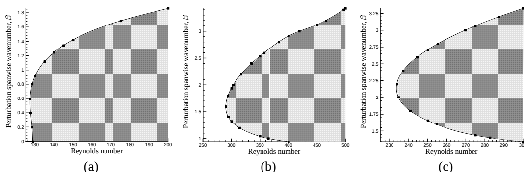
Figure 3. Neutral stability curves: (a) symmetrically constrained flow in symmetric geometry; (b) unconstrained flow in symmetric geometry following primary instability; (c) flow in asymmetric geometry. Shaded regions are linearly unstable.
