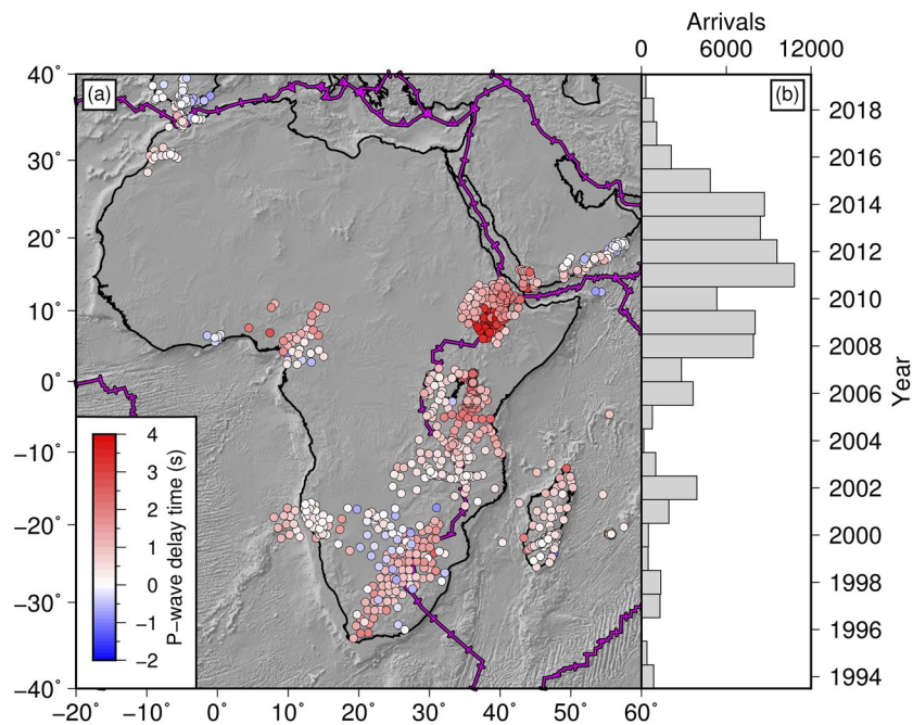
Figure 2. (a) Mean absolute arrival-time residuals for temporary seismic stations across Africa calculated using the absolute arrival-time recovery method (AARM; Boyce et al., 2017) with respect to ak135 (Kennett et al., 1995). Negative residuals are early arrivals (fast); positive residuals are late arrivals (slow). Residuals are corrected for station elevation and plotted on an asymmetric color bar from +4 s to −2 s delay time. Magenta lines: plate boundaries. (b) Histogram of residuals binned by year.
