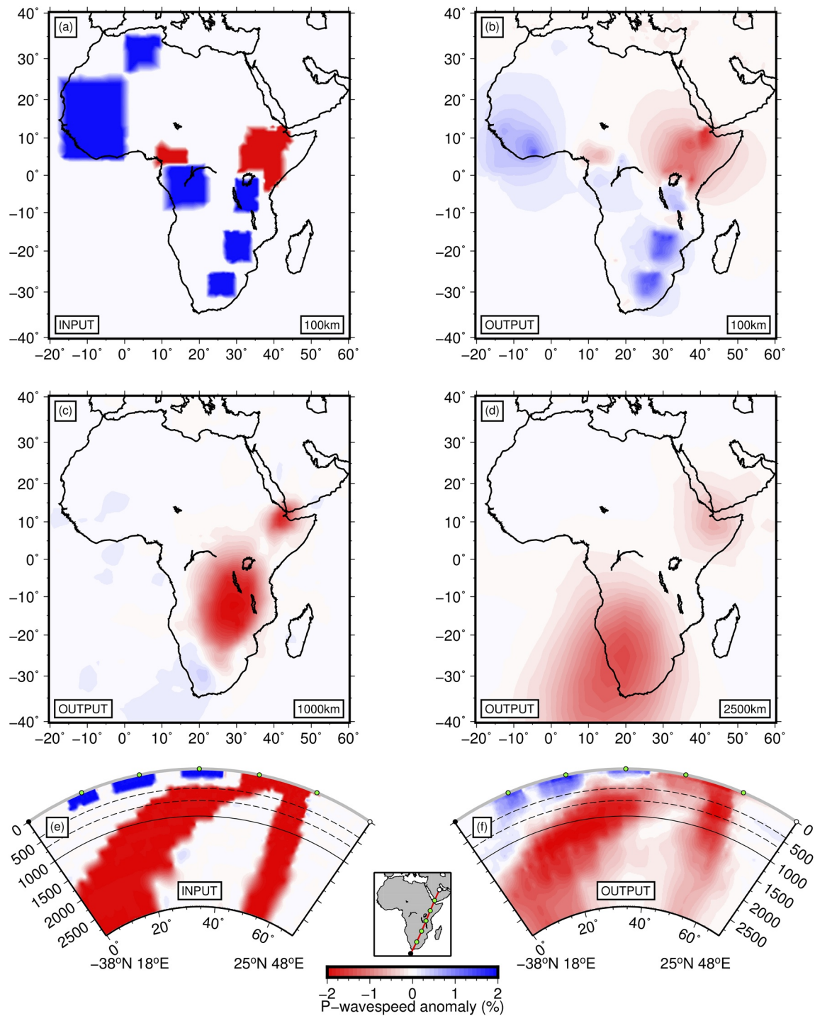
Figure 3. An inclined, elliptical, input slow wavespeed anomaly ( \delta V_P = -2.0\% ) increases in areal extent from the surface, centered at 10^\circ\text{N} , 40^\circ\text{E} , to the core-mantle boundary, centered at 35^\circ\text{S} , 15^\circ\text{E} (a and e). We also add a narrower planform, more steeply dipping slow wavespeed anomaly ( \delta V_P = -2.0\% ) extending from the surface, centered at 10^\circ\text{N} , 42^\circ\text{E} , to the core-mantle boundary, centered at 13^\circ\text{N} , 44^\circ\text{E} (a and e). We insert \delta V_P = +2\% wavespeed anomalies as cratonic cores in the upper 270 km in west Africa, Congo and southern Africa and the upper 180 km in Tanzania. We insert a \delta V_P = -2\% wavespeed anomaly below the Cameroon Volcanic Line to 270 km depth (a and e). We ensure that input whole-mantle slow wavespeed anomalies do not overlap upper mantle input anomalies using a \delta V_P = 0\% buffer region. Visual defects within the input anomaly model result from a coarse adaptive grid in poorly sampled regions. The cross-section location is indicated in the inset map between (e and f). Recovered anomalies, shown at 100, 1,000, 2,500 km depth and in cross-section (b–d, and f) are displayed on the same color scale as the input.
