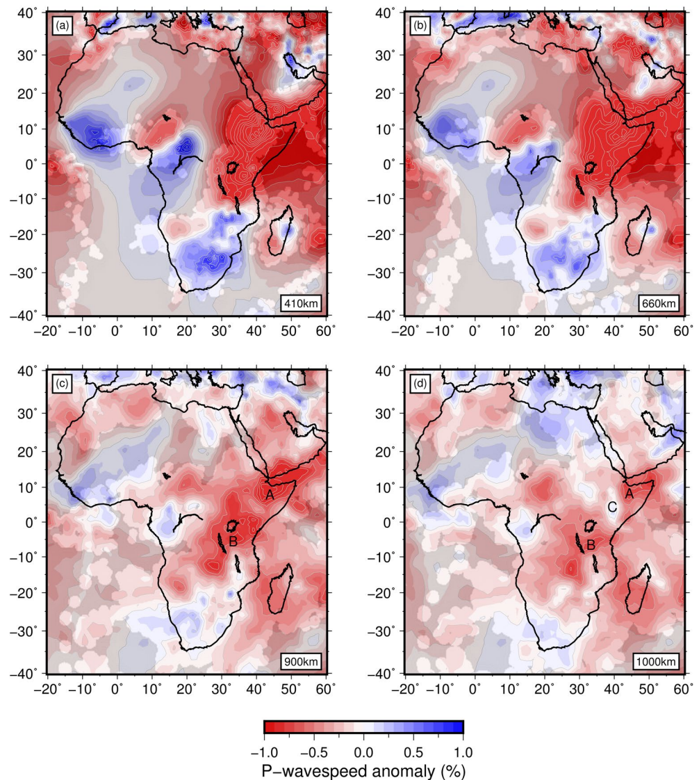
Figure 6. AFRP20 African tomographic model at mid-mantle depths of 410, 660, 900, and 1,000 km (a–d) plotted as percentage deviation from ak135 ( \delta V_p = \pm 1\% ). Gray regions are not constrained by our new AARM-derived African data set (see supporting information), only by the global data set (Li et al., 2008).
