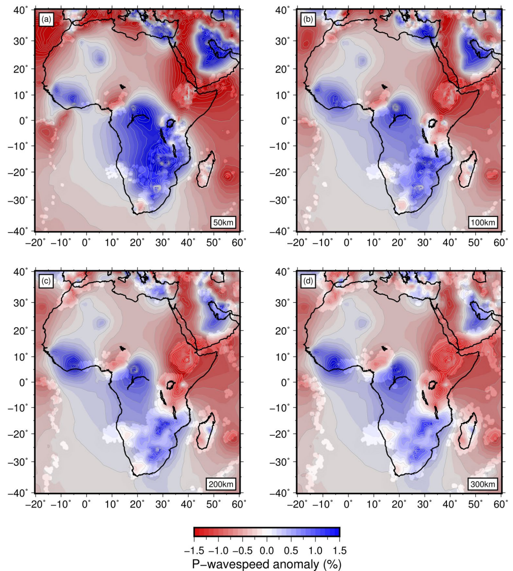
Figure 5. AFRP20 African tomographic model at upper mantle depths of 50, 100, 200, and 300 km (a–d) plotted as percentage deviation from ak135 ( \delta V_P = \pm 1.5\% ). Gray regions are not constrained by our new AARM-derived African data set (see supporting information), only by the global data set (Li et al., 2008). Particularly at these upper mantle depths, resolution offered by the global data set is limited to regions of high earthquake and station density (Figures S1, S2, and S27–S31).
