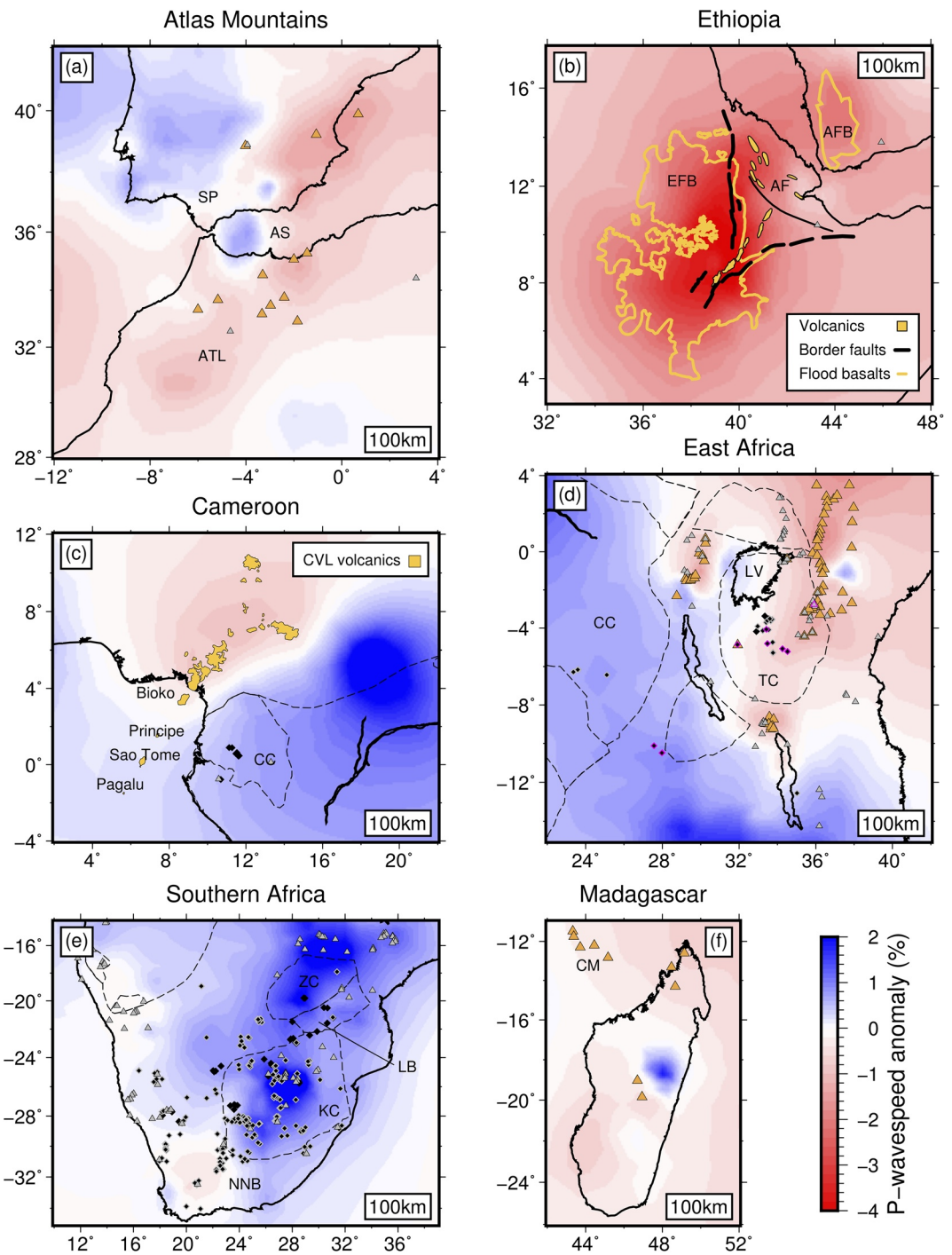
Figure 9. (a–f) P -wavespeeds at 100 km depth within each region for which spatial sampling is greatly improved by the addition of new AARM-derived absolute arrival-times (Figure 2). Orange triangles: Quaternary volcanoes. Gray triangles: Carbonatite volcanoes; the only active Carbonatite volcano at Ol Doinyo Lengai, Tanzania is outlined pink (Woolley & Kjarsgaard, 2008). Black diamonds: kimberlite locations; those erupted since 500 and 50 Ma are outlined in gray and pink, respectively (Tappe et al., 2018). Yellow regions: Cenozoic volcanic provinces. Black dashed polygons: the craton outlines shown in Figure 1. AF, Afar depression; AFB, Arabian flood basalts; AS, Alboran Sea; CM, Comoros and Mayote; EFB, Ethiopian flood basalts; LV, Lake Victoria. Other acronyms follow Figure 1. Wavespeed plotted as percentage deviation from ak135 on an asymmetric color scale ( -4\% \leq \delta V_p \leq 2\% ) to illuminate the full extent of wavespeed heterogeneity.
