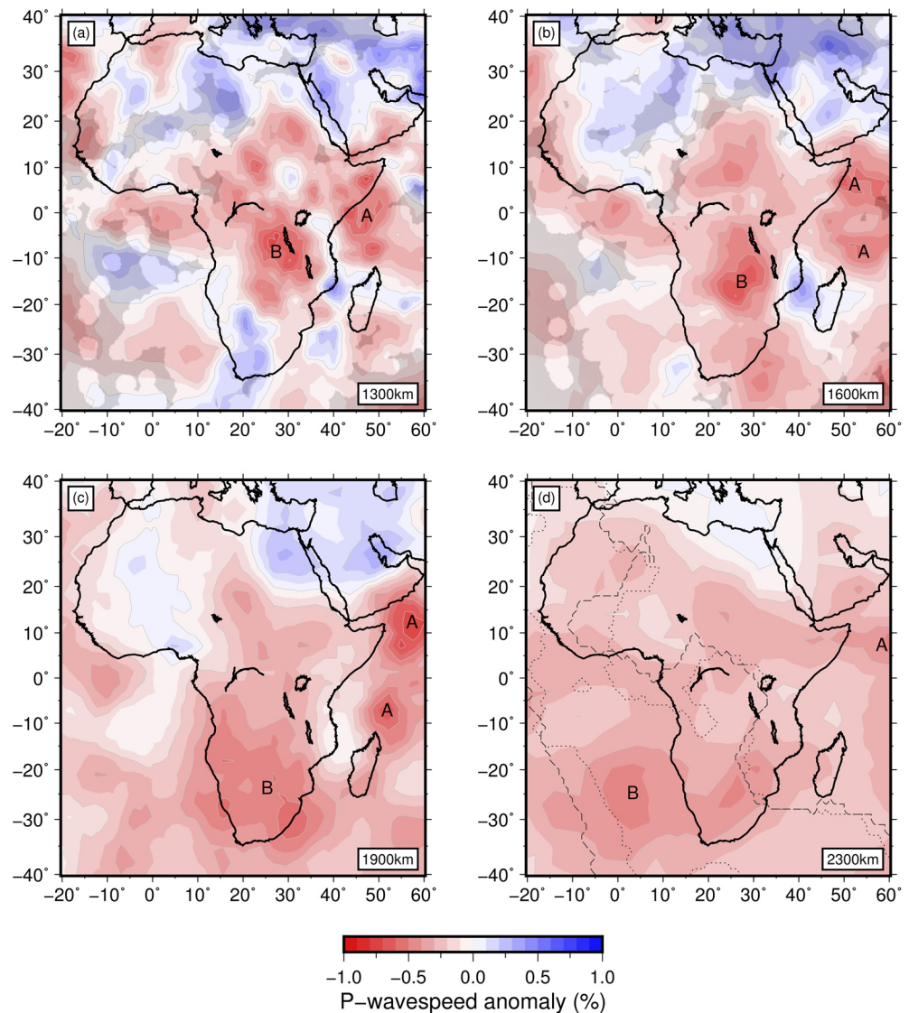
Figure 7. AFRP20 African tomographic model at lower mantle depths of 1,300, 1,600, 1,900, and 2,300 km (a–d) plotted as percentage deviation from ak135 ( \delta V_P = \pm 1\% ). Gray regions are not constrained by our new AARM-derived African data set (see supporting information), only by the global data set (Li et al., 2008). Within subplot (d), dashed and dotted dark gray lines mark regions of 5/5 slow-wavespeed votes near the core-mantle boundary in \delta V_S and \delta V_P tomographic models respectively, clustered by Cottaar and Lekić (2016). Anomaly B lies inside these contours while anomaly A lies outside.
