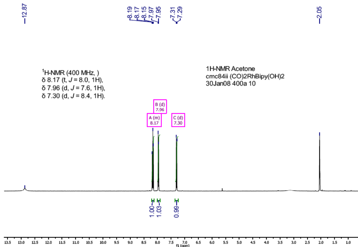
Figure S3. 1 H NMR spectrum of complex [Rh( 2 )(CO) 2 ]SbF 6 in CD 3 COCD 3 at 298 K.
