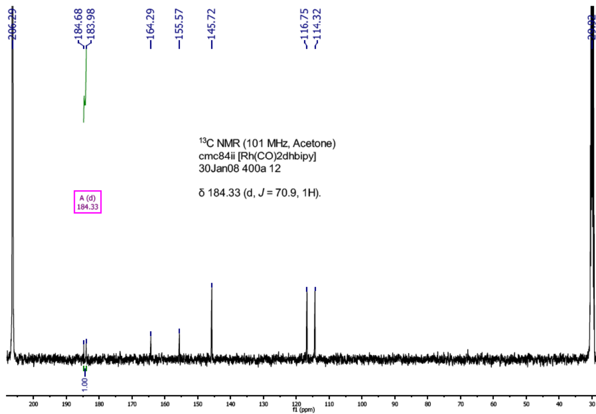
Figure S4. 13 C{ 1 H} NMR spectrum of complex [Rh( 2 )(CO) 2 ]SbF 6 in CD 3 COCD 3 at 298 K.
