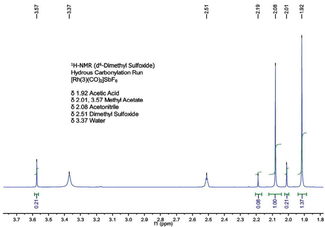
Figure S10. Example of product analysis by 1 H NMR for carbonylation experiment under aqueous conditions.
