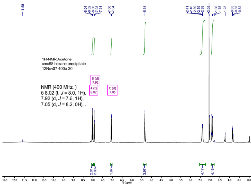
Figure S2. ^1\text{H} NMR spectrum of complex [\text{Rh}(\mathbf{2})(\text{cod})]\text{SbF}_6 in \text{CD}_3\text{COCD}_3 at 298 K.
