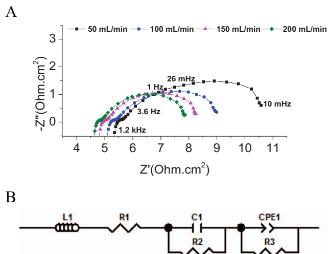
Figure 6. A) Nyquist representation of the EIS response of the whole cell at different vanadium flow rates with a hydrogen flow rate of 100 mL/min. B) Equivalent circuit used to fit the EIS data where L1 = L , R1 = R_s , C1 = C_{dl} , R2 = R_{CT} , CPE1 = CPE and R3 = R_{Diff} .
