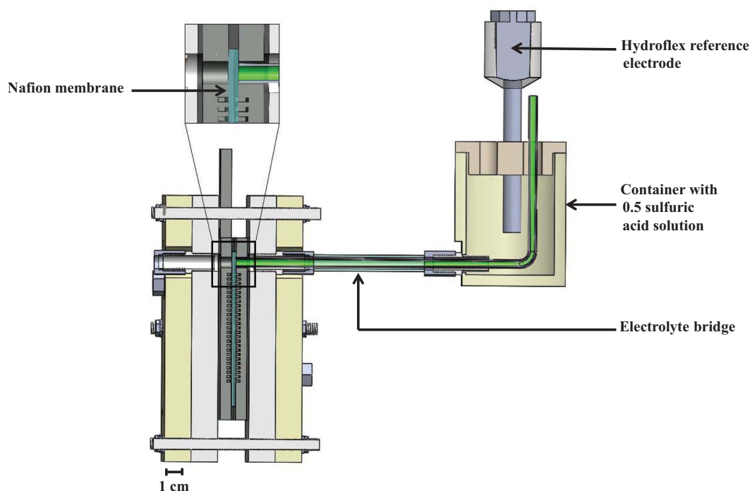
Figure 1. Schematic of the assembled RHVFC with the integration of the reference electrode set-up (Figure Credit: A. Kavei).
