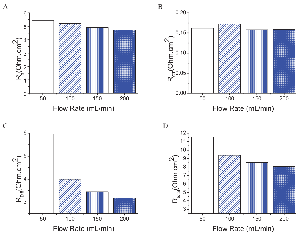
Figure 7. A) Series B) Hydrogen charge transfer C) Vanadium diffusion D) Total resistance of the whole cell at different vanadium flow rates and at 100 mL/min hydrogen flow rate.
