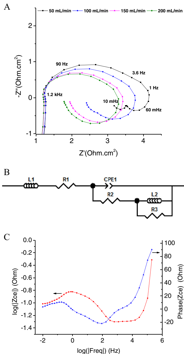
Figure 4. A) Nyquist representation of the EIS response of the hydrogen half-cell at different vanadium flow rates with a hydrogen flow rate of 100 mL/min. B) Equivalent circuit used to fit the EIS data where L1 = L_{wires} , R1 = R_s , CPE1 = CPE , R2 = R_{ads/des} , L2 = L_{ads\_Pt} , R3 = R_{ads\_Pt} . C) Bode plots of the EIS response of the hydrogen half-cell at different vanadium flow rates with a hydrogen flow rate of 100 mL/min.
