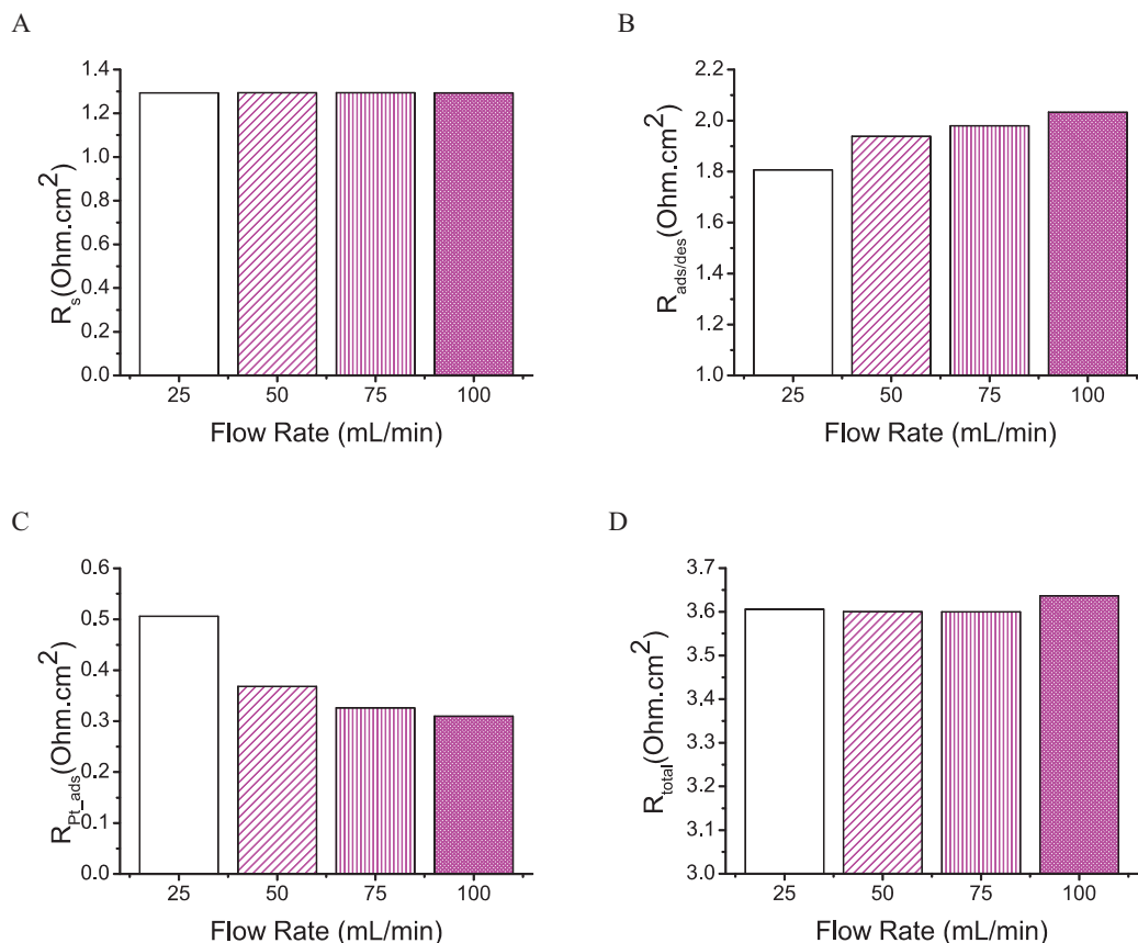
Figure 8. A) Series B) Hydrogen adsorption/desorption C) Vanadium adsorption D) Total, resistance of the anode at different hydrogen flow rates and at 100 mL/min vanadium flow rate.
