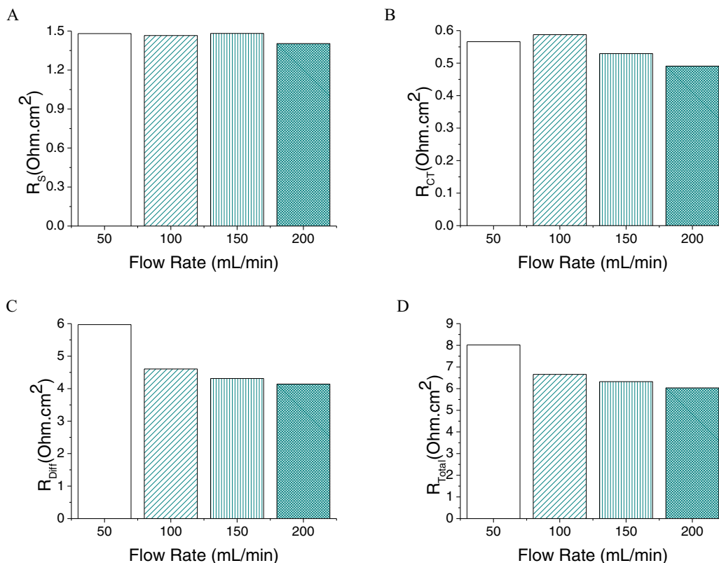
Figure 3. A) Series B) Charge transfer C) Diffusion D) Total, resistance of the cathode at different vanadium flow rates and at 100 mL/min hydrogen flow rate.
