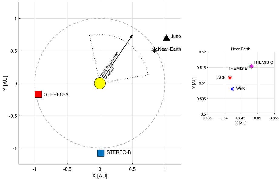
Figure 1 Location of the near-Earth spacecraft (ACE, Wind, and ARTEMIS), Juno, STEREO-A and STEREO-B on 25 October 2011 at 00:00 UT in Heliocentric Aries Ecliptic (HAE) coordinates. Imagery on board the STEREO spacecraft can be used to estimate the initial propagation direction and extent of the ICME, represented by the black arrow and dotted lines, respectively (for details, see Section 3). The near-Earth spacecraft are in near radial alignment with Juno, with a small maximum longitudinal separation of 3.6^\circ . The inset shows a close up of the configuration of the near-Earth spacecraft: ACE (red), Wind (blue), THEMIS B (green) and THEMIS C (magenta). The near-Earth spacecraft configuration has a maximum radial separation of < 0.01 AU and a maximum longitudinal separation of < 0.2^\circ .
