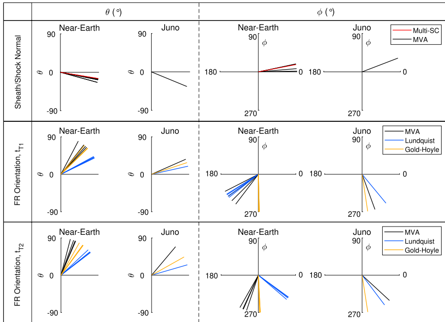
Figure 6 Calculated orientations presented in RTN coordinates, where \theta is the angle to the R - T plane, and \phi is the angle swept out anticlockwise from the Sun–Earth line, projected onto the R - T plane ( \phi = 180^\circ points sunwards). \theta is presented for the near-Earth spacecraft and Juno in the first column, and \phi is presented for the near-Earth spacecraft and Juno in the second column. The normal directions to the sheath calculated using MVA (black) and the propagation direction of the shock calculated using timing considerations between the near-Earth spacecraft (red) are presented in the first row. The flux rope orientations calculated by MVA (black), Lundquist (blue), and Gold–Hoyle fitting (orange) using the earlier trailing edge are presented in the second row, and in the third row using the later trailing edge.
