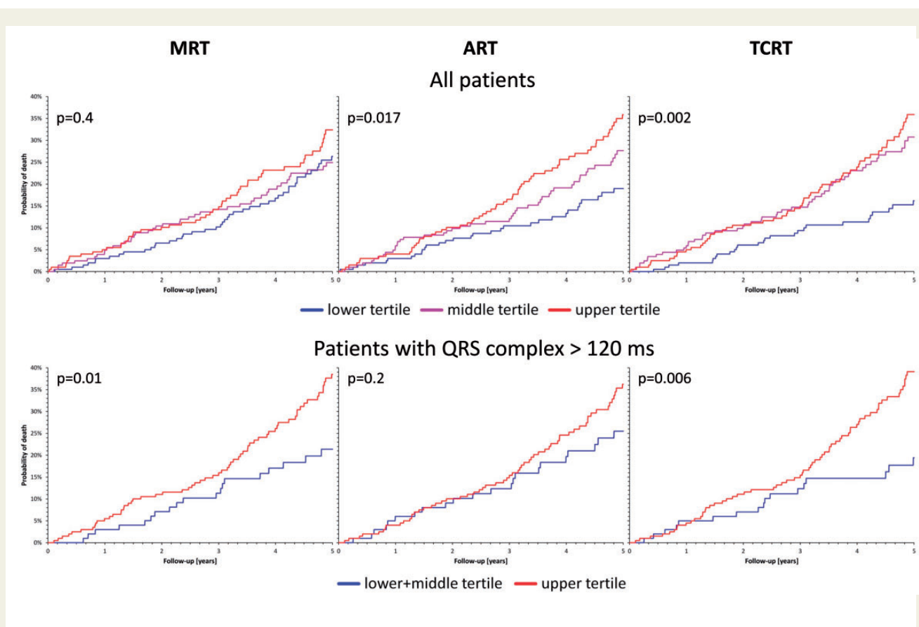
Figure 5 Probabilities of death during follow-up of ICD recipients. Kaplan–Meier curves show the probability of death during follow-up among the recipients of implantable defibrillators stratified according to the spatial QRS-T angle. For each graph, the P -value of the \chi^2 (top row) and log-rank (bottom row) test comparison of the probabilities is also shown. The top and bottom rows correspond to the complete population and to patients with QRS complex width > 120 ms. In the top row, the blue, violet, and red curves correspond to patients with QRS-T angles within the smallest, middle, and largest tertile of the measurements. In the bottom row, the blue and red curves correspond to patients with the QRS-T angles within the smallest and the two larger tertiles of the measurements, respectively. The left, middle, and right column correspond to the prediction based on the maximum R to T (MRT), area R to T (ART), and total cosine R to T (TCRT) calculations, respectively.
