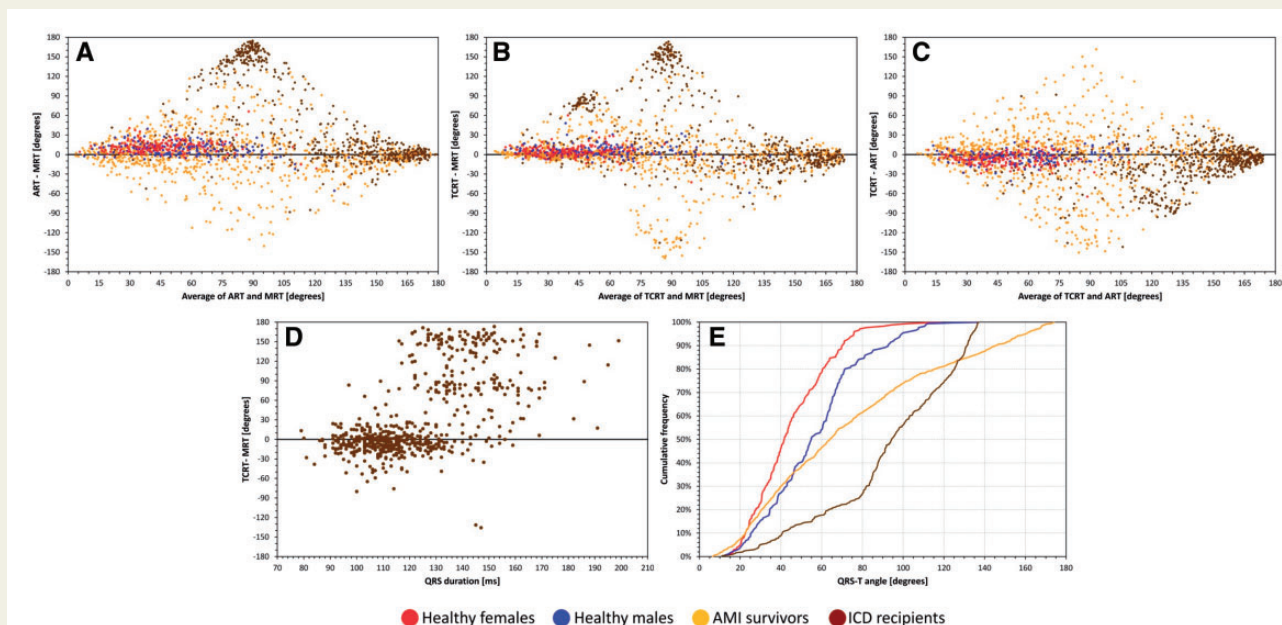
Figure 1 Comparisons of QRS-T angle measurements. Panels A–C show the differences between the different methods for QRS-T angle calculation obtained for individual subjects and patients (see the text for details). Panel D shows the relationship of the differences between the TCRT and MRT methods in dependency on the QRS complex duration which is used as a surrogate of QRS loop abnormality. Panel E shows the cumulative distributions of the TCRT assessment of the QRS-T angle in different populations. Note that in panels A–C, the trapezoidal shape of the graphs is determined by the fixed range of all measurements between 0 and 180° (e.g. the maximum difference of 180° between two measurements can only exist if one measurement is 0 and the other 180°). The red, blue, yellow, and brown marks and lines correspond to healthy females, healthy males, survivors of acute myocardial infarction, and recipients of implantable defibrillators (ICD), respectively. (Note that panel D shows the data for the ICD recipients.) MRT, maximum R to T; ART, area R to T; TCRT, total cosine R to T; ICD, implantable cardioverter defibrillators (see the text for explanations).
