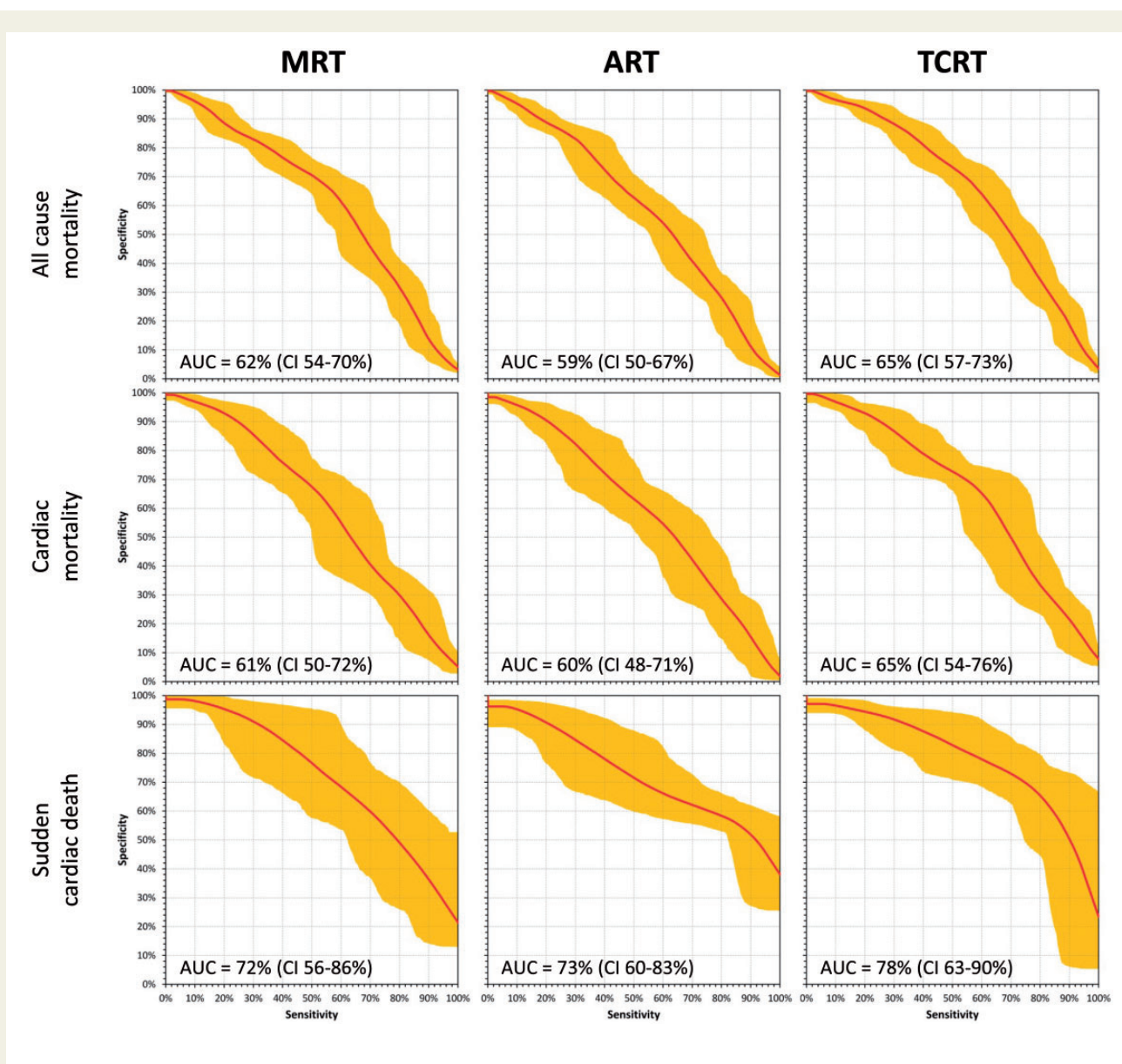
Figure 3 Prediction of outcome in survivors of acute myocardial infarction. The figure shows receiver operator characteristics for the prediction of outcome events among survivors of acute myocardial infarction based on increased values of the spatial QRS-T angle. The graphs show the median curvatures and their 90% confidence bands obtained by bootstrap (see the text for details). The top, middle, and bottom row correspond to the prediction of all-cause mortality, cardiac death, and sudden cardiac death, respectively. The left, middle, and right column correspond to the prediction based on the maximum R to T (MRT), area R to T (ART), and total cosine R to T (TCRT) calculations, respectively. Numerical values of the areas under the characteristics (AUC) and of their 90% confidence intervals (CI) are shown in each panel (see also Table 2).
