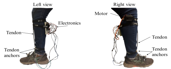
Fig. 1. Side views of the prototype of the proposed low-cost assistive ankle device worn on the right leg with both the circuit and motor shown. The tendon is attached to an anchor point above the shoelaces and at another point at the ankle before attaching to the motor worn on the shin.
