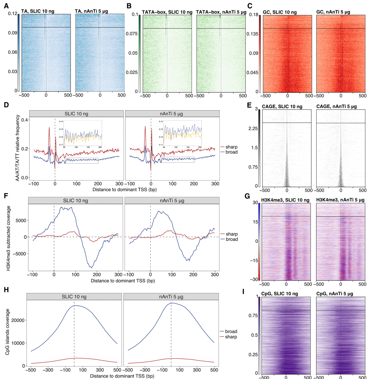
Figure 4. SLIC-CAGE is equivalent to nAnt-iCAGE for pattern discovery. Comparison of SLIC-CAGE derived from 10 ng and nAnt-iCAGE derived from 5 µg of M. musculus total RNA. In all heat maps, promoters are centered at the dominant CTSS (dashed vertical line at 0) and ordered by tag cluster inter-quantile width with sharpest promoters on top and broadest on the bottom of each heat map. The horizontal line separates sharp and broad promoters (empirical boundary for sharp promoters is set at inter-quantile width \leq 3 ). (A) Comparison of TA dinucleotide density in the SLIC-CAGE (left) and nAnt-iCAGE library (right). As expected, sharp promoters have a strong TA enrichment, in line with the expected TATA-box in sharp promoters around the -30 position. (B) Comparison of TATA-box density in SLIC-CAGE (left; 14.3% of TCs have a TATA-box around -30 position) vs. nAnt-iCAGE library (right; 14.5% of TCs have a TATA-box around -30 position). Promoter regions are scanned using a minimum of the 80th percentile match to the TATA-box position weight matrix (PWM). Sharp promoters exhibit a strong TATA-box signal as suggested in A. (C) Comparison of GC dinucleotide density in the SLIC-CAGE (left) and nAnt-iCAGE library (right). Broad promoters show a higher enrichment of GC dinucleotides across promoters, suggesting the presence of CpG islands, as expected in broad promoters. (D) Average WW (AA/AT/TA/TT) dinucleotide frequency in sharp and broad promoters identified in SLIC-CAGE (left) or nAnt-iCAGE library (right). Inset shows a closer view on WW dinucleotide frequency (blue) overlain with the signal obtained when the sequences are aligned to a randomly chosen identified CTSS within broad promoters (yellow). Ten-base-pair WW periodicity implies the presence of well-positioned +1 nucleosomes in broad promoters, in line with the current knowledge on broad promoters. (E) Tag cluster coverage heat map of SLIC-CAGE (left) or nAnt-iCAGE library (right). Signal enrichment in broad promoters indicates well-positioned +1 nucleosomes, in line with the presence of WW periodicity in broad promoters. (F) H3K4me3 relative coverage in sharp versus broad promoters identified in SLIC-CAGE (left) or nAnt-iCAGE (right). (G) H3K4me3 signal density across promoter regions centered on SLIC-CAGE or nAnt-iCAGE-identified dominant CTSS. (H) Relative coverage of CpG islands across sharp and broad promoters, centered on the dominant CTSS identified in SLIC-CAGE (left) or nAnt-iCAGE (right). These results agree with GC-dinucleotide density signal, which is much stronger in broad promoters. (I) CpG islands coverage signal across promoter regions centered on the dominant CTSS identified in SLIC-CAGE (left; 68.1% of TCs overlap with a CpG island) or nAnt-iCAGE (right; 64.4% of TCs overlap with a CpG island).
