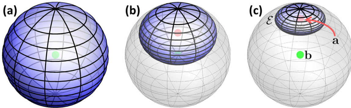
Figure 3. The geometric data for three maximal volume states \tilde{\rho}_c^{\max} with (a) c = 0 , (b) c = 0.5 and (c) c = 0.8 . Since these are canonical states we have \tilde{\mathbf{b}} = \mathbf{0} and \mathbf{c} = \mathbf{a} . Note that \mathcal{E} = \mathcal{E}_c^{\max} touches the North pole of the Bloch sphere for any c .
