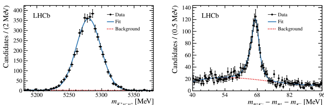
Figure 2. Distributions of normalization candidates in (left) mass, m_{K^+ \mu^- \mu^+} , and (right) the mass difference, m_{B^+ K^-} - m_{B^+} - m_{K^-} . The result of each fit is shown as a solid line, with the background component as a dashed line.
