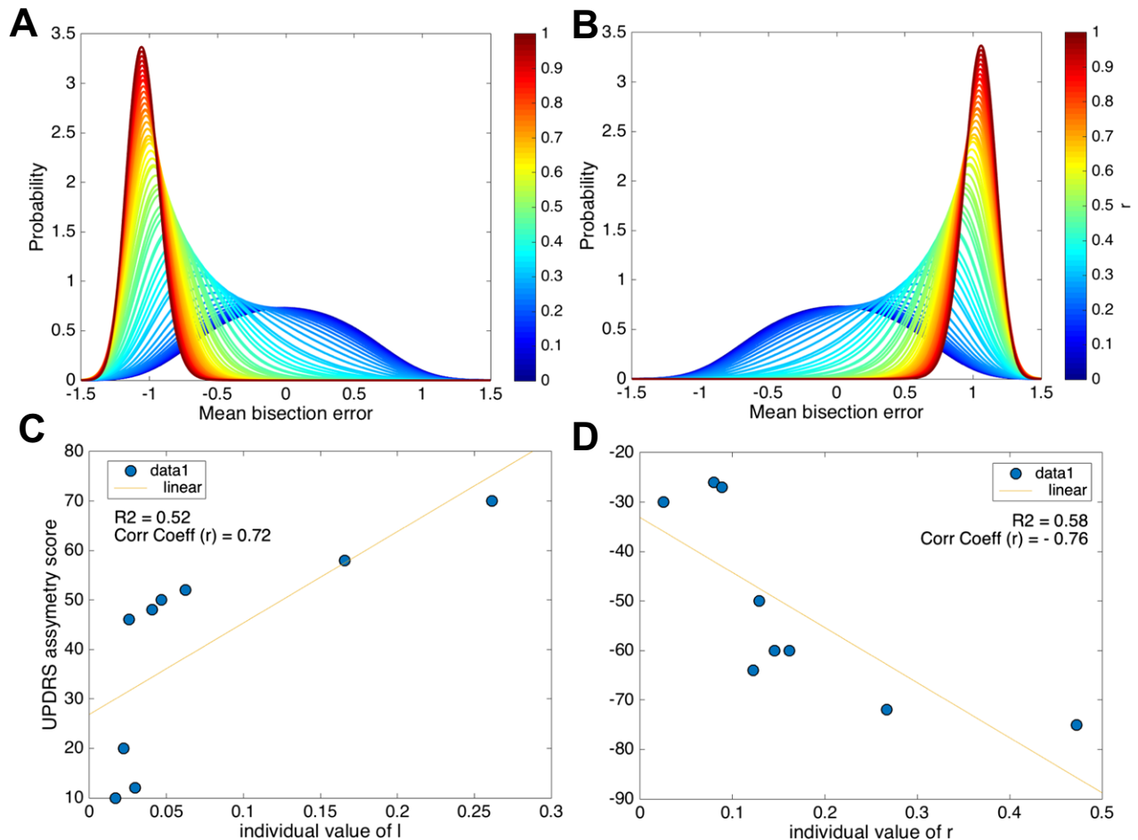
Figure 4. Computational Model: (A and B) Figure illustrates the probability distribution p(x; l, r) that occurs for several different values of l (A) or r (B) where the following fixed parameters were implemented in the model r or l = 5.0 and \beta = 1 . (C and D) relationship between calculated values of l (RPD) (4C) and r (LPD) (4D) and UPDRS asymmetry. Note two patients (one RPD and one LPD) were excluded as they were outliers.
