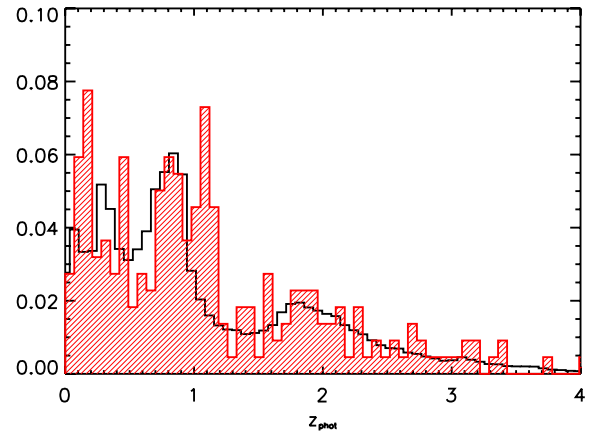
Figure 12. Photometric redshift distribution in the CDFS field (in normalized counts). The black histogram shows the distribution of all objects in the SWIRE survey field, the red shaded one is the distribution of objects along the line of sight of the Planck clump. While the spikes at z < 1 reflect the overall redshift distribution in the NDWFS field, a peak at z \sim 1.1 is only found along the line of sight of the clump.
