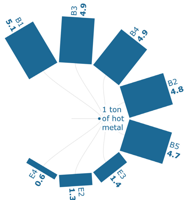
Figure 3c. FPMF of iron (PM 2.5 eq./FU). Fine Particulate Matter Formation of iron (PM 2.5 eq./Functional Unit). Please refer to Table 2 for the descriptions of the scenarios.
