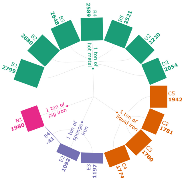
Figure 3b. GWI of iron (kg CO 2 eq./FU). Global Warming Impact of iron (kg CO 2 eq./Functional Unit). Please refer to Table 2 for the descriptions of the scenarios.
