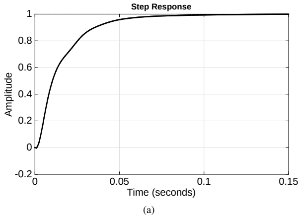
Fig. 6: Step response of different PLLs
