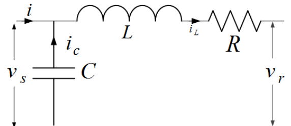
Fig. 4: \Gamma section representing cable, transformer and converter impedance
