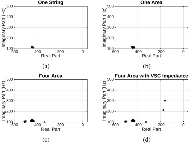
Fig. 10: Subsystems's oscillatory modes in the 100 Hz to 500 Hz range
