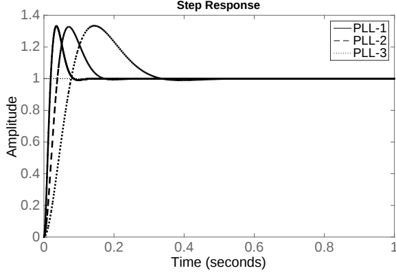
Fig. 6: Step response of different PLLs
