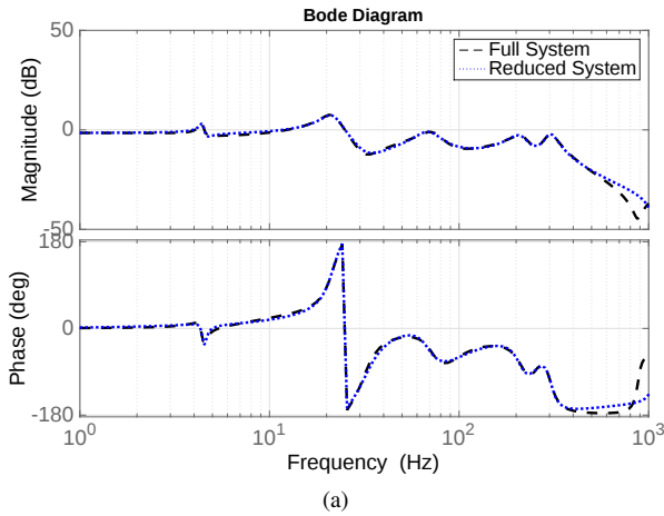
Fig. 13: Bode diagram comparing transfer function of the full wind farm system and 12 th order reduced system
