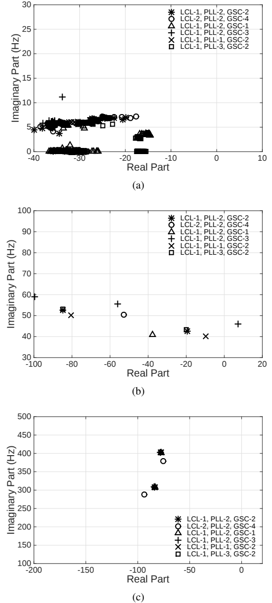
Fig. 14: Closed loop eigenvalues using different LCL filters, GSC controllers, and PLLs
