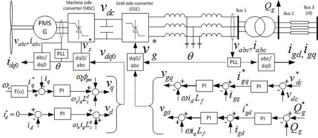
Fig. 2: PMSG SMIB system
