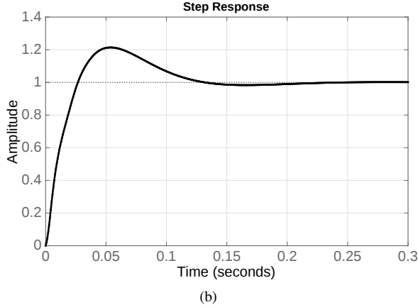
Fig. 7: Step response of GSC (a) reactive power and (b) capacitor voltage control loop
