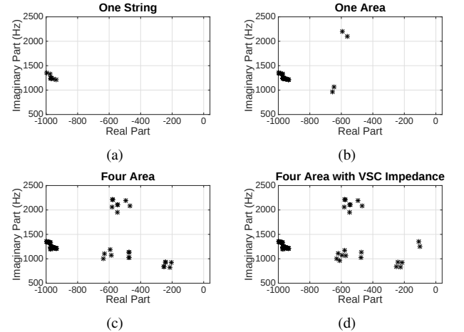
Fig. 9: Subsystems's oscillatory modes in the 500 Hz to 2.5 kHz range
