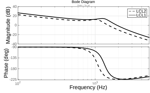
Fig. 5: LCL filter bode of transfer function i_g/v_i
