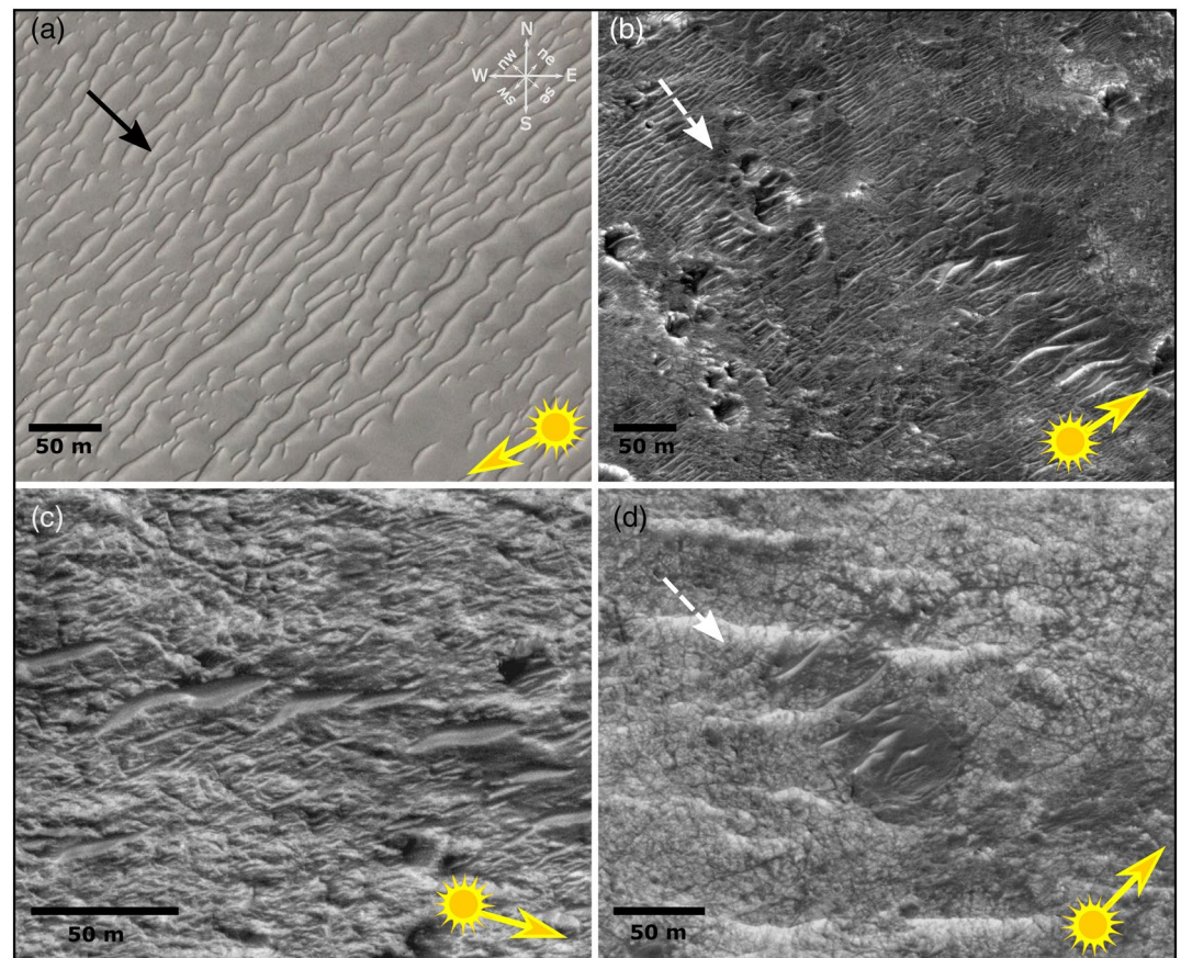
Figure 10. There are morphological and albedo similarities between (a) megaripples in the Argentinian Puna (26°36'35.51"S, 67°34'06.04"E) and (b)–(d) Oxia Planum (ESP_041422_1985, PSP_009735_1985, ESP_040433_1985, respectively). Using the grainsize-albedo relationship confirmed by E. Favaro et al. (2020) in Argentina, the stoss and lee slopes of TARs in Oxia Planum can be identified. This allows for characterization of the winds necessary to result in these orientations. The sun angle at time of image acquisition is also noted, demonstrating these albedo relationships are present in terrestrial and martian megaripples and TARs, respectively, irrespective of sun angle. TAR, Transverse Aeolian Ridges.
