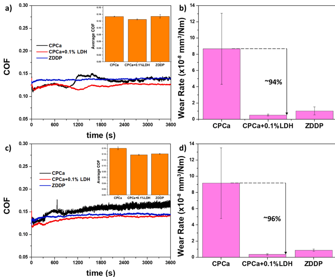
Fig. 5. Friction coefficient (a) and average wear rate (b) of CPCa, CPCa + 0.1%LDH, and ZDDP lubricants under 10 N at 50°C. Friction coefficient (c) and average wear rate (d) of CPCa, CPCa + 0.1%LDH, and ZDDP lubricants under 10 N at 100°C.
