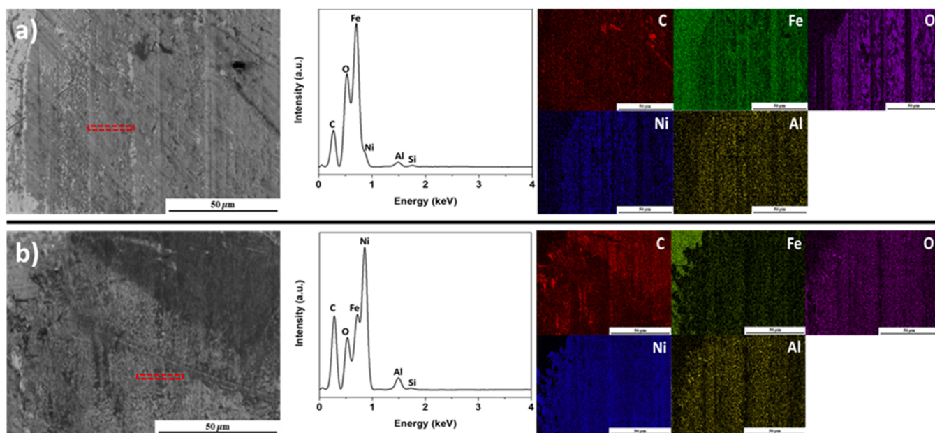
Fig. 6. SEM and EDS results of the ball wear scar surfaces lubricated by CPCa + 0.1%LDH under 10 N at (a) 50^\circ\text{C} and (b) 100^\circ\text{C} . (The red rectangles in (a) and (b) indicating the areas for FIB milling).
