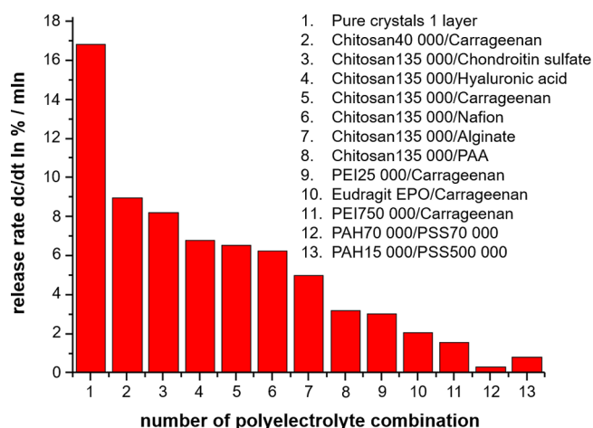
Figure 7. Permeability of layer-by-layer (LbL) membranes consisting of different polyelectrolyte combinations (8 layers) for small molecules (fluorescein). Unpublished data from the group of Lars Dähne.
