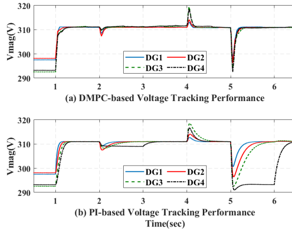
FIGURE 15 Voltage control performance with cyber and physical events.
