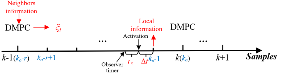
FIGURE 5 Time-sequence cooperation between the event-triggered DMPC and the non-asymptotic observer.
