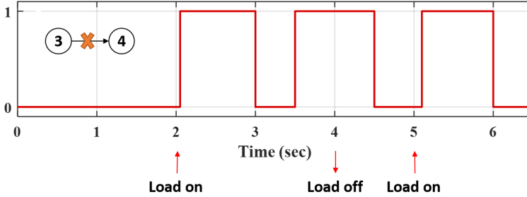
FIGURE 14 Physical and cyber events of the 4-DG MG system: value "1" represents that the communication channel between DG3 and DG4 is unavailable; the load change occurs at 2s, 4s and 5s respectively.
