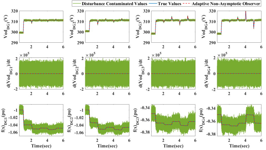
FIGURE 8 Non-asymptotic observer performance (base value of f(x) : 7.35 \times 10^9 ).
