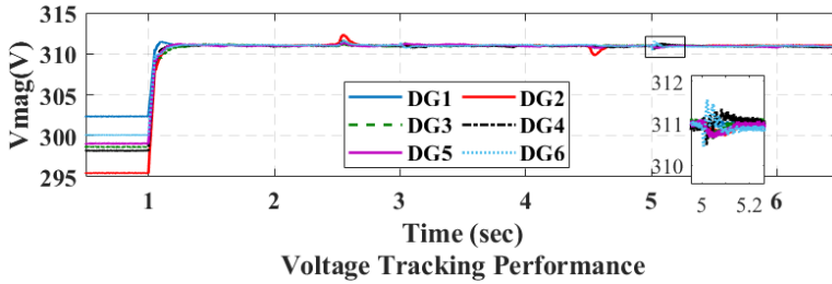
FIGURE 19 Voltage control performance with system reconfiguration in the modified IEEE-13 bus system
