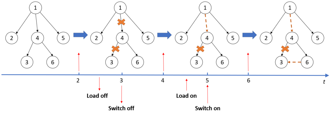
FIGURE 18 Physical and cyber events of modified IEEE-13 bus MG system
