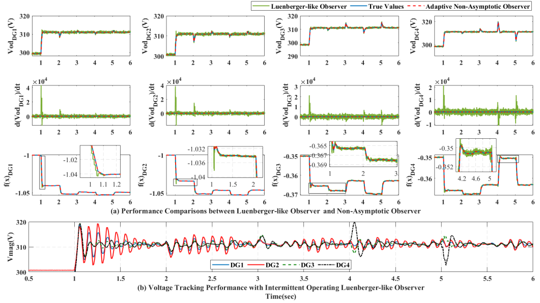
FIGURE 9 Voltage control performance with intermittent operating Luenberger-like observer.
