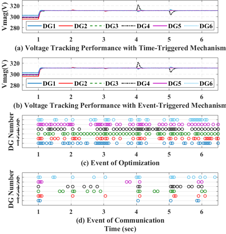
FIGURE 17 Voltage control performance of modified IEEE-13 bus MG system: (a) voltage tracking performance with time-triggered mechanism; (b) voltage tracking performance with event-triggered mechanism; (c) event-triggered time of DMPC optimization; (d) event-triggered time of neighbouring communication.
