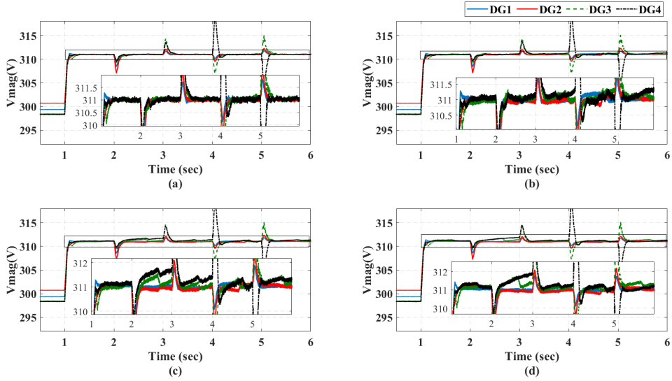
FIGURE 11 Event-triggered condition with fixed e_{com} ( e_{com} = 0.1 ) but different thresholds e_{opt} : (a) e_{opt} = 0.05 ; (b) e_{opt} = 0.1 ; (c) e_{opt} = 0.15 ; (d) e_{opt} = 0.2 .
