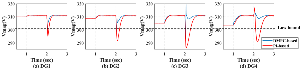
FIGURE 10 Voltage control performance under the extreme condition.
