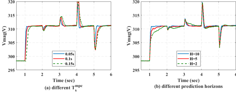
FIGURE 13 Effects of information update frequency and prediction horizon.
