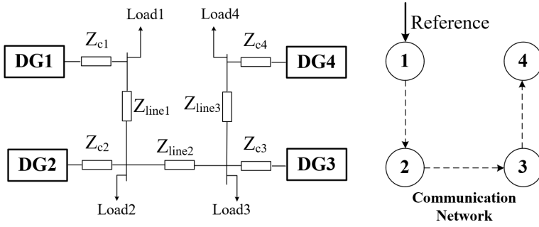
FIGURE 6 Diagram of the tested 4-bus MG system.
