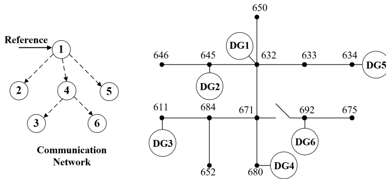
FIGURE 16 Diagram of modified IEEE-13 bus MG system
