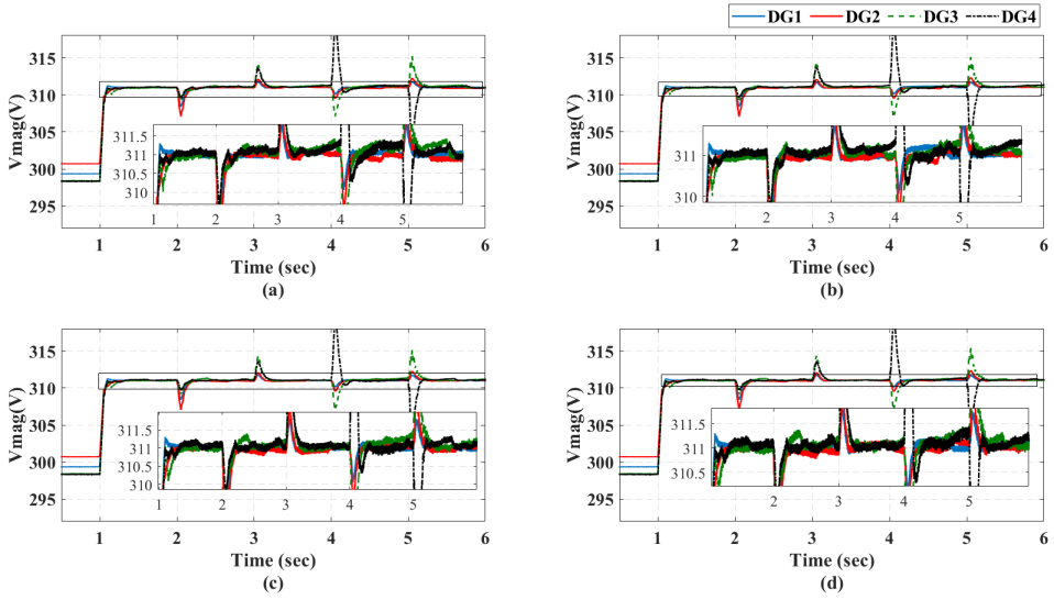
FIGURE 12 Event-triggered condition with fixed e_{opt} ( e_{opt} = 0.1 ) but different thresholds e_{com} : (a) e_{com} = 0.05 ; (b) e_{com} = 0.1 ; (c) e_{com} = 0.15 ; (d) e_{com} = 0.2 .
