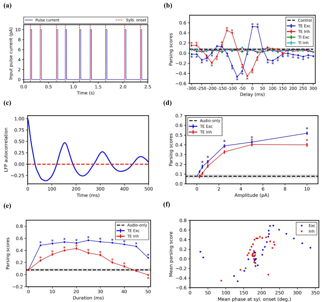
Figure 2. Effect of a pulse input current on the parsing scores. (a) An example of an excitatory pulse input current signal with the onsets of the pulses located at the syllable onsets. (b) An excitatory input to the excitatory neurons (blue) can both improve the syllable parsing or impede it, depending on the delay. A positive delay hereby means that the pulses occur after the corresponding syllable onset. An inhibitory current to the excitatory neurons can influence the syllable parsing as well (red). Neither excitatory (green) nor inhibitory (cyan) current projected to the inhibitory neurons, however, has a significant effect on the syllable parsing. (c) The autocorrelation of the LFP in the absence of a speech stimulus or a visual current shows a periodicity of about 150 ms. (d) The mean parsing scores as a function of the amplitude of the pulse current. The excitatory inputs (blue) occur at 25 ms after the syllable onsets whereas the inhibitory input (red) is presented 125 ms before the syllable onset. (e) The mean parsing scores as a function of the duration of the pulse current. The excitatory inputs (blue) are presented 25 ms after the syllable onsets whereas the inhibitory input (red) occurs 125 ms before the syllable onset. (f) The mean parsing score is optimal for a particular phase of the LFP at the syllable onset, both for the excitatory current (blue) and for the inhibitory current (red). Statistical significance is denoted by asterisks ( p < 0.05 , FDR correction for multiple comparisons).
