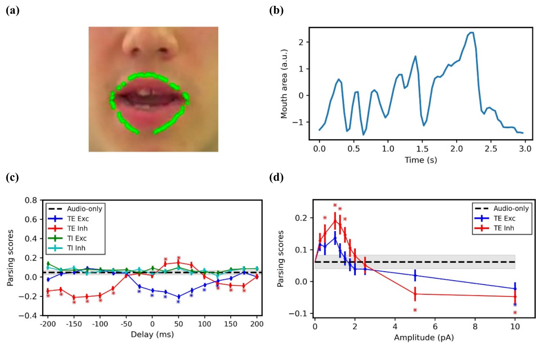
Figure 3. Effect of a current proportional to the mouth-opening area on the parsing scores. (a) The area of mouth opening is derived from the contour of the lips (green) (b) The area is then computed for every image in a video and z-scored to yield the time-varying mouth-opening area. (c) Adding an excitatory (blue) current to the excitatory neurons could significantly worsen the parsing score, whereas an inhibitory current (red) could both improve and worsen it. In contrast, neither an excitatory nor an inhibitory current presented to the inhibitory neurons had an impact on the parsing scores (green and cyan). (d) The mean parsing scores as a function of the amplitude of the visual current. The excitatory input (blue) is presented 125 ms preceding the auditory input whereas the inhibitory input (red) is added at a delay of 50 ms. Statistical significance is denoted by asterisks ( p < 0.05 , FDR correction for multiple comparisons).
