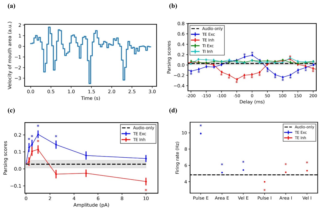
Figure 4. Effect of a current based on the velocity of the mouth-opening area on the parsing scores. (a) An example current signal. (b) Presenting an excitatory current (blue) or an inhibitory current (red) to the excitatory neurons could, at certain delays, significantly improve the parsing score as compared to no visual input (black). However, adding either an excitatory or inhibitory current to the inhibitory neurons (cyan and green) did not influence the syllable parsing. (c) The mean parsing scores as a function of the amplitude of the visual current. The excitatory inputs (blue) were presented at a delay of -25 ms, whereas the inhibitory input (red) was added at a delay of 125 ms. (d) The firing rates of the excitatory neurons under the different conditions. The excitatory pulse inputs (Pulse E) were presented at a delay of 25 ms, whereas the inhibitory pulse inputs (Pulse I) occurred at a delay 125 ms. The excitatory current corresponding to the mouth-opening area (Area E) was presented at a delay of -125 ms whereas the corresponding inhibitory current input (Area I) occurred at a delay of 50 ms. The excitatory current corresponding to the velocity of the mouth-opening area (Vel E) was added at a delay of -25 ms whereas the corresponding inhibitory current (Vel I) occurred at a delay of 125 ms. All input currents cause significantly different firing rates in the excitatory neurons, and in particular for the case of the excitatory pulse inputs (Pulse E). Statistical significance is denoted by asterisks ( p < 0.05 , FDR correction for multiple comparisons).
