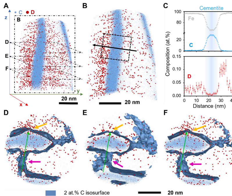
Fig. 6. Hydrogen maps of hydrogen-desorbed strained steel specimen. (A) is a reconstructed 3-dimensional atom map, where carbon (C) and deuterium (D) atoms are shown in blue and in red, respectively. (B) is a 10-nm-thick slice view of the region in the y-z plane marked by the black dashed lines in (A). (C) provides the elemental concentrations of iron (grey), carbon (blue), and deuterium (red) from the 30 nm x 40 nm cylindrical ROI marked by the black dashed lines in (B). (D–F) are 5-nm-thick slices from the x-y planes marked by the dashed lines in (A), using 2 atomic percent carbon isosurfaces to highlight the carbon-rich regions.
