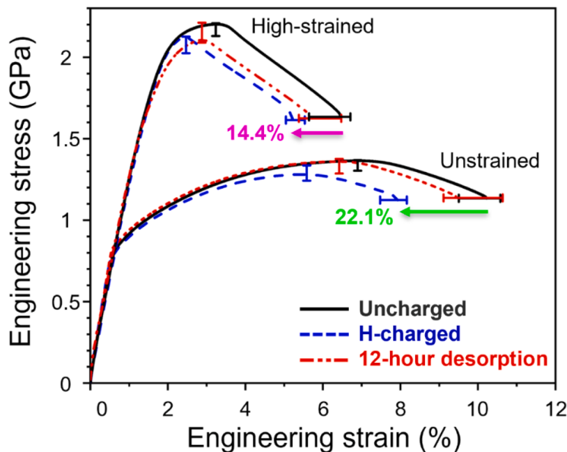
Fig. 4. SSRT stress-strain curves of high-strained and unstrained specimens for hydrogen embrittlement susceptibility. Black, blue, and red refer to uncharged, hydrogen-charged and tested immediately (H-charged), and hydrogen-charged desorbed for 12 hours at room temperature in vacuum (12-hour desorption). The error bars refer to ultimate tensile strength and elongation, which are obtained from 3 data points for each condition.
