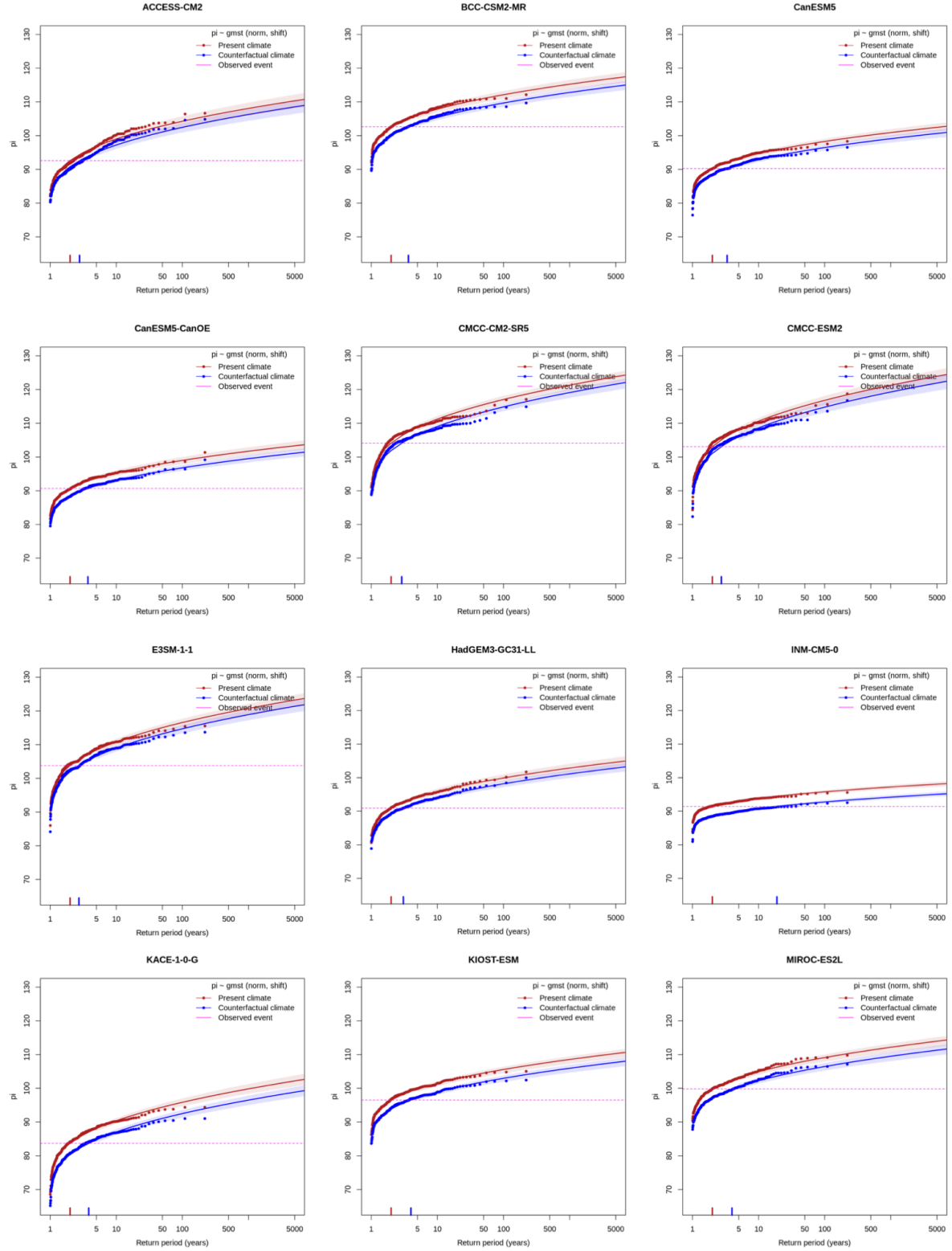
Figure A.3: Return level plots for CMIP6 models. The influence of GMST is shown in the difference between the red vs blue probability curves and the magnitude of the event is highlighted with a purple line (right). Part 1.
