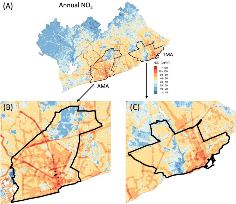
Figure 4. Estimated (A) annual NO 2 in the GAMA with zoom in for (B) AMA and (C) TMA.
