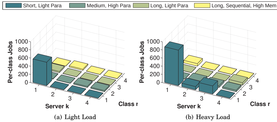
Fig. 12. Optimized Placement of Workload under light and heavy Load
