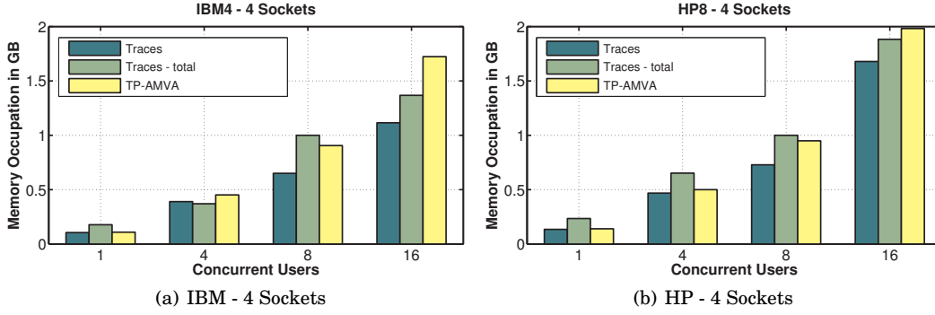
Fig. 11. Predicted Peak Memory Occupation under Multi-User Scenario (normalized by the "Traces - total" value from 8 User Scenario)
