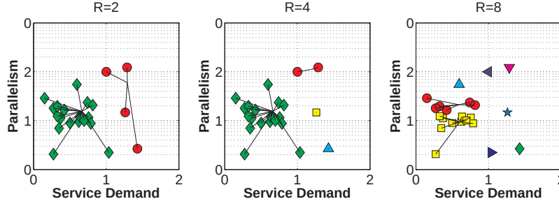
Fig. 16. Normalized Query Classes for different Numbers of k-means Clusters (logarithmic scaling)
