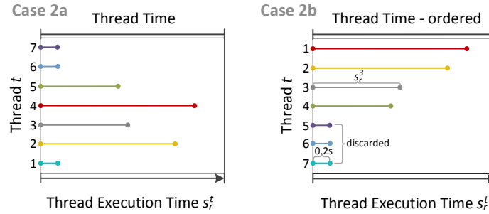
Fig. 15. Service Demand Estimation for an OLAP Query
