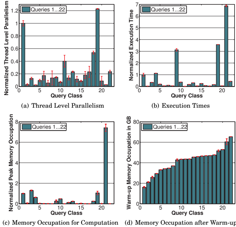
Fig. 3. OLAP Workload Characteristics (normalized by respective value of Query Class 1)
