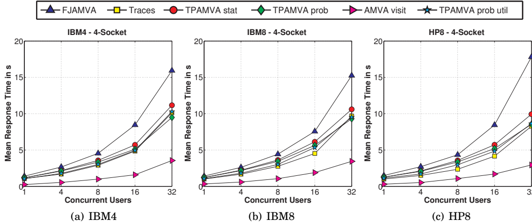
Fig. 9. Predicted Response Times across different Hardware Types with 4 Sockets (normalized by Response Times from 4-Socket Con 1 Scenario on IBM8)
