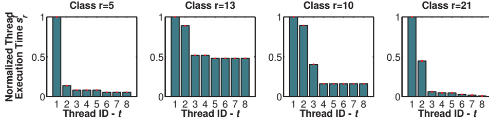
Fig. 5. Thread Times for the 8 longest running threads of respective class r .
