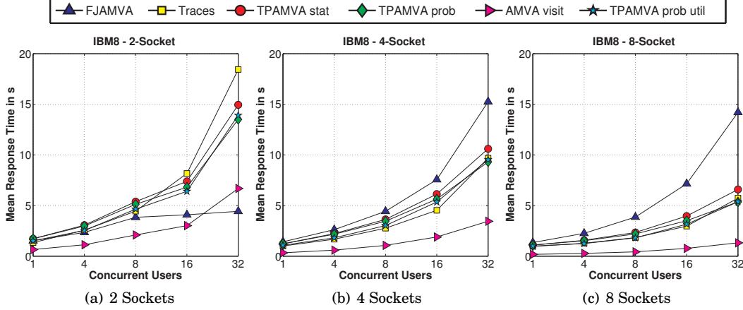
Fig. 8. Predicted Response Times across different NUMA Configurations on the IBM 8-Socket System (normalized by Response Times from 4-Socket Con 1 Scenario on IBM8)
