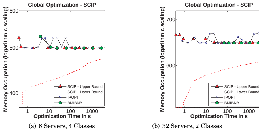
Fig. 17. Global Optimization (stopped after 6% Duality Gap reached)
