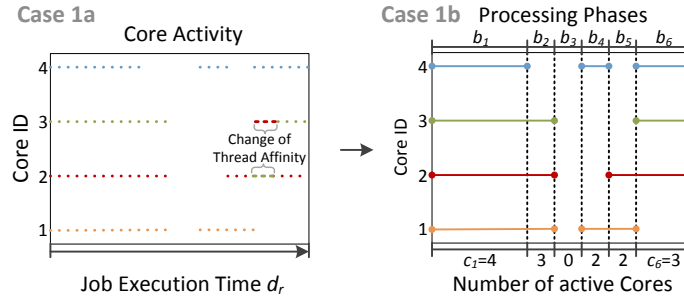
Fig. 6. Service Demand Estimation for an OLAP Query
