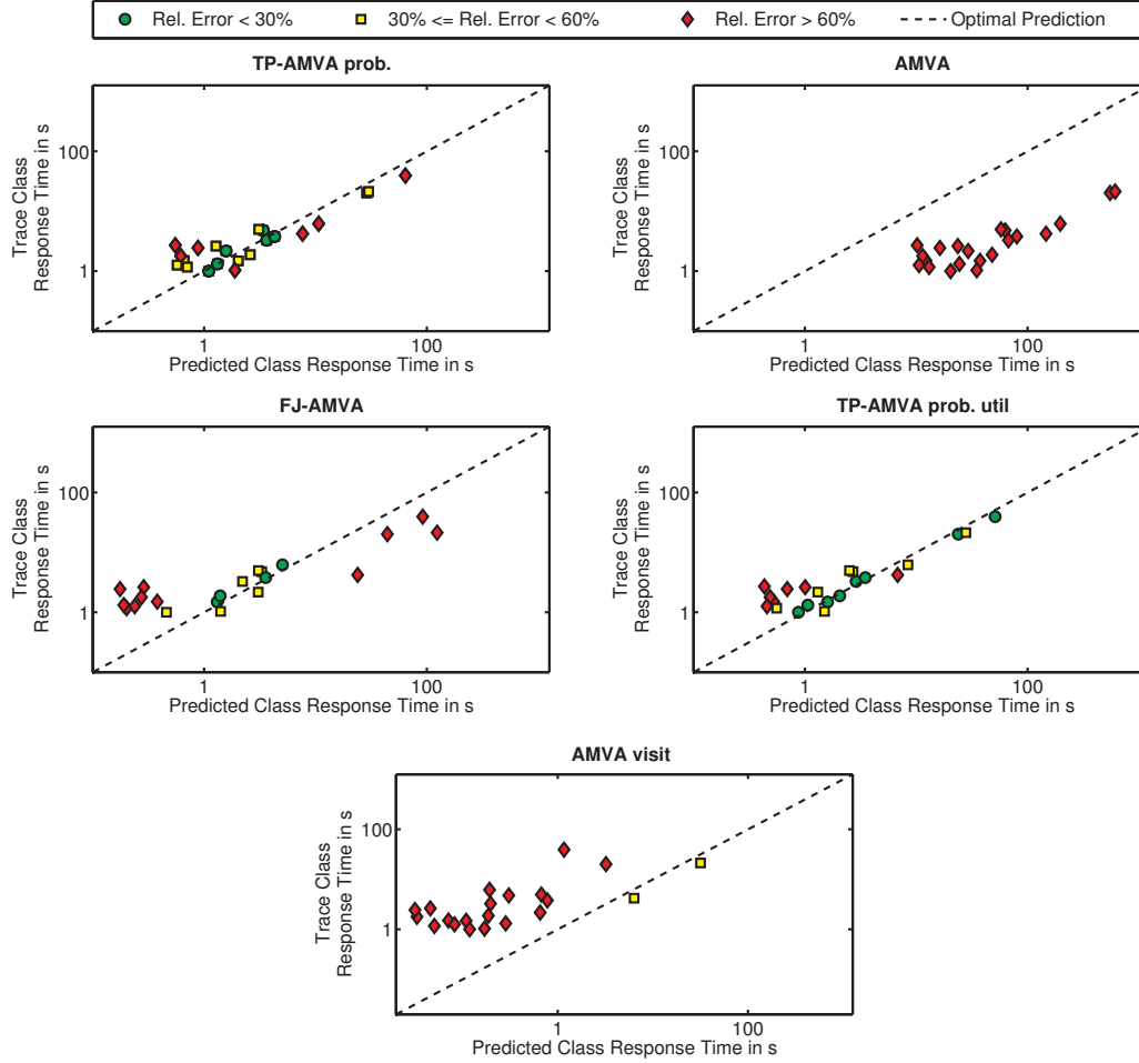
Fig. 7. Comparison of predicted per-class Response Times with per-class Trace Response Times from 8 User Scenario on the IBM4 4-socket default NUMA Configuration (normalized by Response Times of Class 1)
