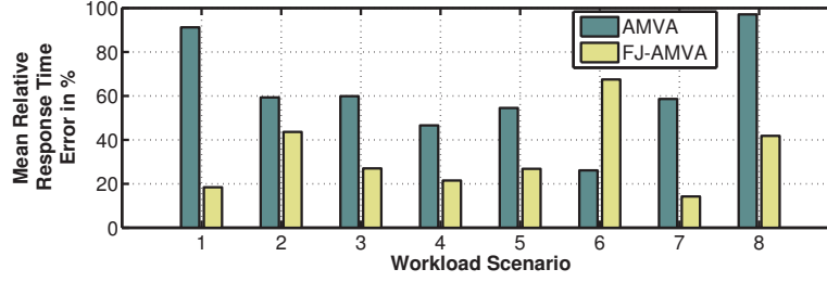
Fig. 1. Predicted Response Time Error vs. Simulation
