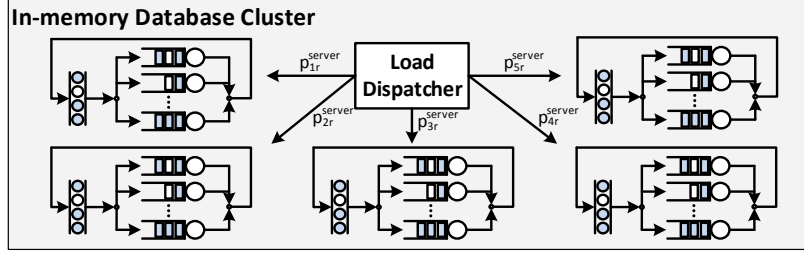
Fig. 10. Model of an in-memory Cluster Subject to Load Optimization
