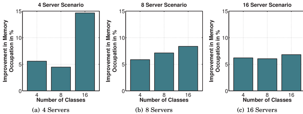
Fig. 14. Improvement in simulated Memory Occupation using optimal Workload Placement found by TP-AMVA prob util compared with TP-AMVA prob as baseline
