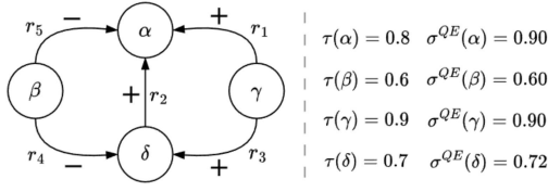
Figure 7: LLMs example.
