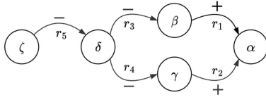
Figure 2: An example of QBAF (where all base scores are set to 0.5).
