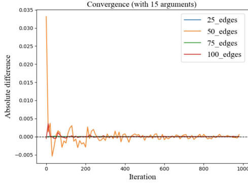
Figure 4: Convergence of Algorithm 1 for random cyclic QBAFs with 15 arguments and various numbers of edges.
