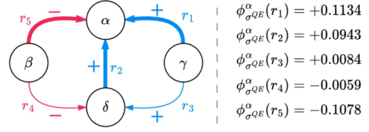
Figure 8: Contributions and RAEs for the LLMs example .
