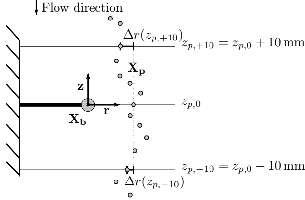
Figure 7: Illustration of the radial deviation, \Delta r(z_p) of a tracer particle trajectory, \mathbf{X}_{p,c} = (r_p, \theta_p, z_p)^T , around a bubble, \mathbf{X}_b . Hereby, the radial deviation is defined as the distance between the reference point, z_{p,0} , and the comparison point, z_{p,+10} or z_{p,-10} . The comparison points, z_{p,+10} and z_{p,-10} , mark the particle position 10 mm upstream and downstream of the bubble, respectively.
