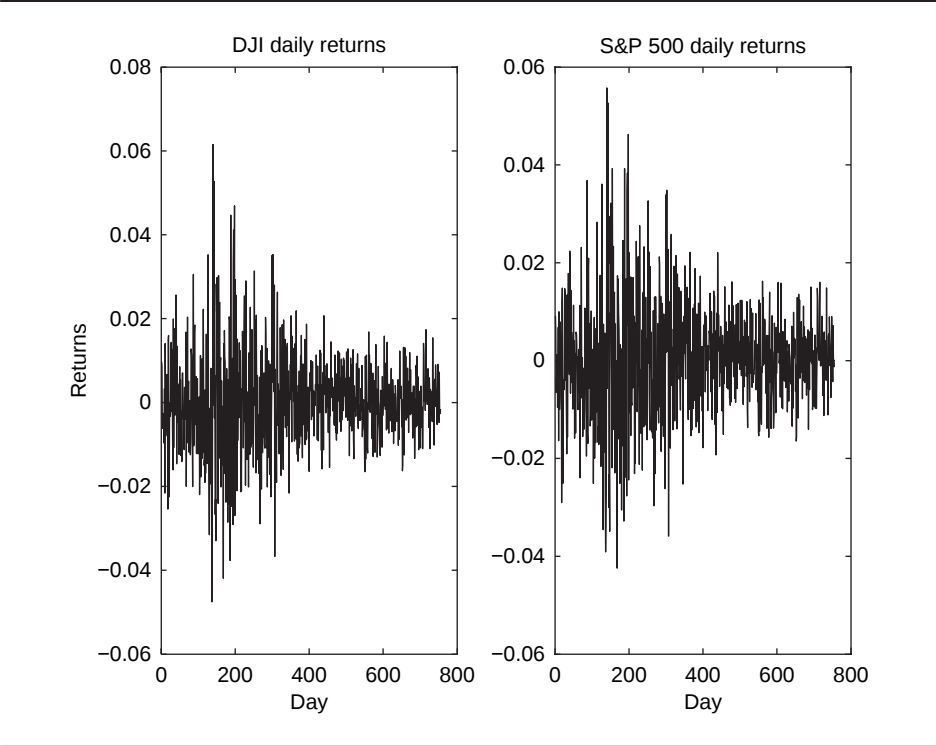
FIGURE 3 Log-returns time series for the Dow Jones index (DJI) and the S&P 500 index.
