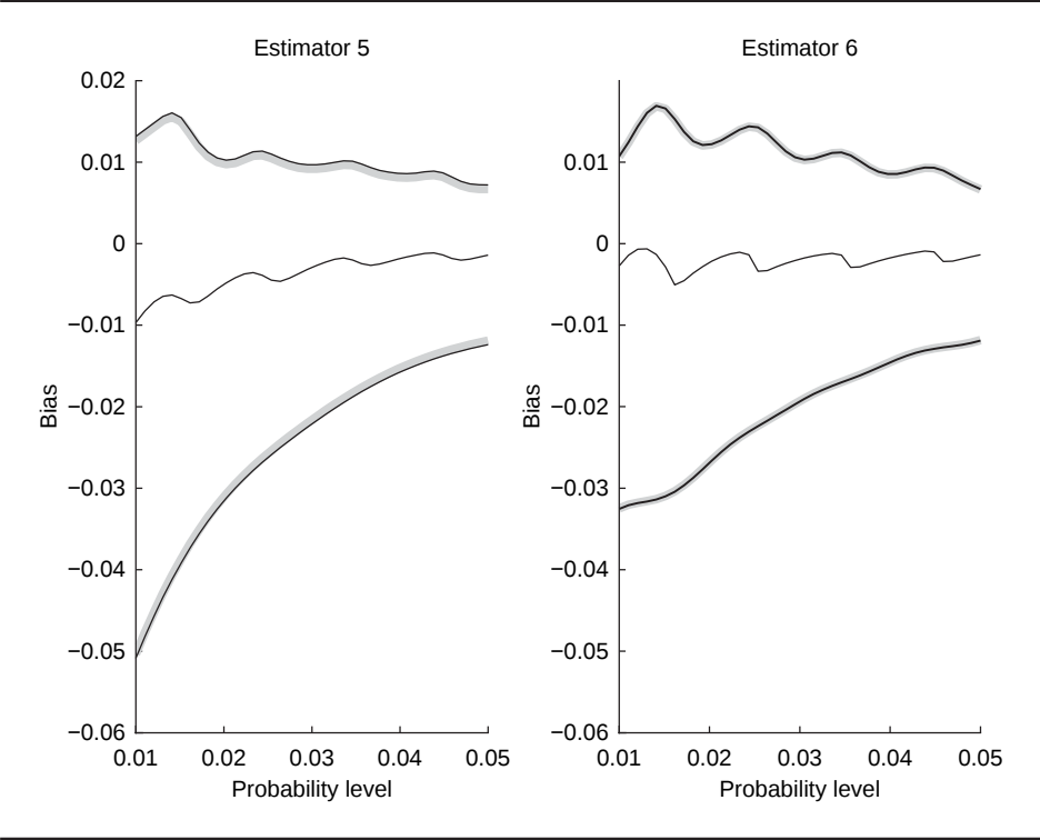
FIGURE 1 The estimated bias together with 95% confidence bands for Est5(1S)_{order} (left panel) and Est6(1S)_{br(5)} (right panel), based on model 1 with n = 100 .
