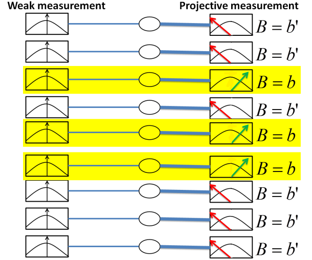
FIG. 1: An illustration of the operational protocol. The particles are all prepared in the same initial state. They are first measured weakly by measurement devices shown on the left, followed by a projective measurement of observable B shown on the right. The shift in the mean position of the measurement devices that weakly interacted with the particles on the postselected set (shaded) corresponding to outcome b has terms proportional to the real and imaginary parts of the weak value.
