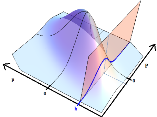
FIG. 2: Joint probability distribution of the momenta of the particle and measurement device after weak measurement. The position p of the particles are weakly measured with devices sampled from a momentum distribution with mean zero and \Delta_P \neq 0 . Each particle's momentum is shifted by an amount proportional to the momentum of the device P , following (34). If one now postselects measurement devices based on the particle having momentum p = b , then the distribution of these devices is shown on the plane intersecting the plot. The mean of this postselected distribution is no longer zero.
