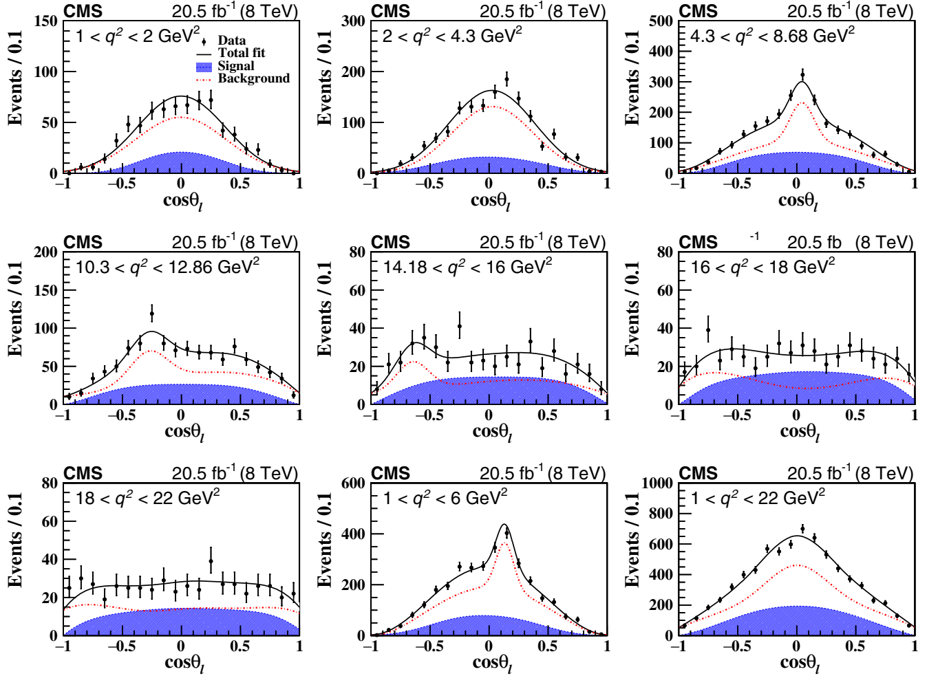
FIG. 4. Projections of the \cos \theta_\ell distributions for each q^2 range from the two-dimensional fit of data. The solid lines show the total fit, the shaded area the signal contribution, and the dashed-dotted lines the background. The vertical bars on the points represent the statistical uncertainty in the data.
