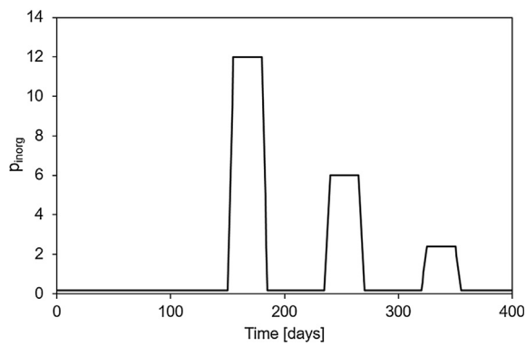
Fig. 2. Inorganic-to-organic proportionality ratio ( p_{ionrg} ) over the operation period considered.
