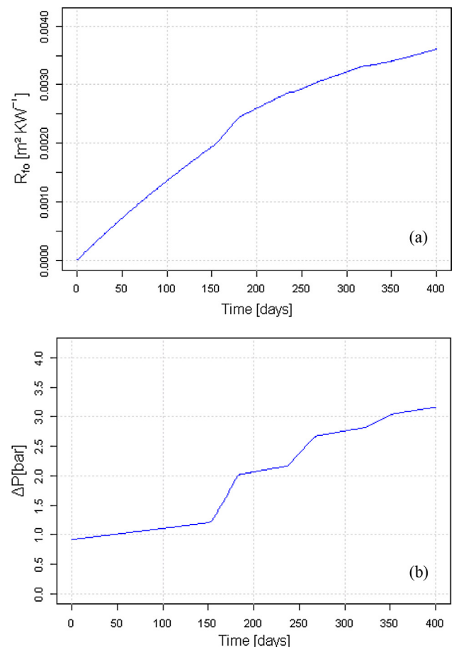
Fig. 8. Average fouling thermal resistance (a) and tube-side pressure drop (b) over 400 days of operation with intermittent inorganic breakthrough episodes.
