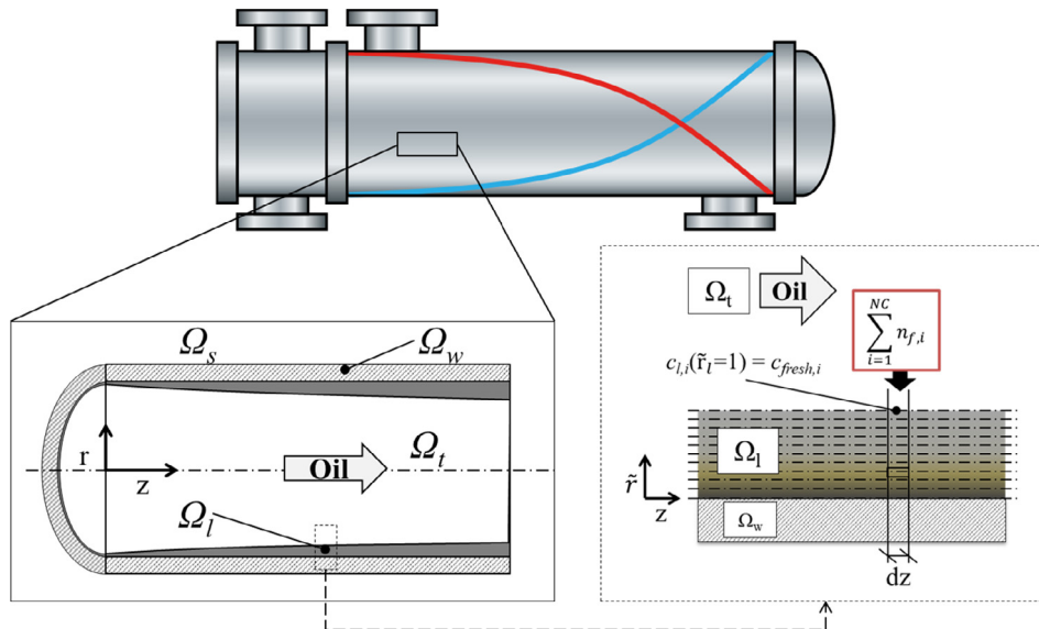
Fig. 1. Schematic representation of a growing fouling layer at a particular location along a heat exchanger tube within a shell-and-tube heat exchanger (adapted from Diaz-Bejarano et al. [28]).
