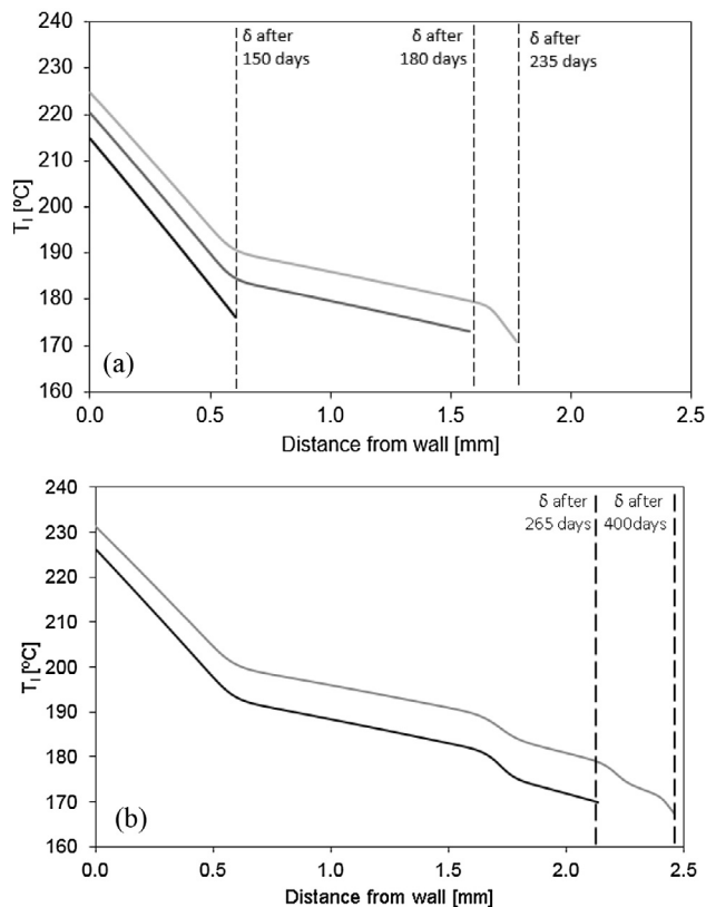
Fig. 7. Radial temperature profile in the deposit, at the exit of the 2nd pass of shell B, at the end of the operation period: after 150, 180 and 235 days (a); after 265 and 400 days (b).
