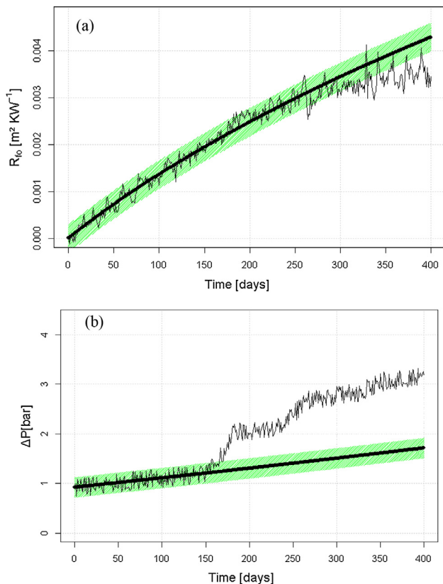
Fig. 9. Average fouling thermal resistance (a) and tube-side pressure drop (b) for expected baseline behavior (thick line; called predicted line) and scenario with intermittent inorganic breakthrough episodes (thin line; called monitored line). The green band indicates the uncertainty of the baseline prediction.
