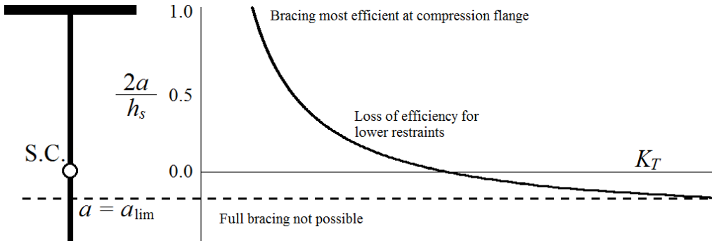
Figure 7: The effect of restraint height on bracing ability.
