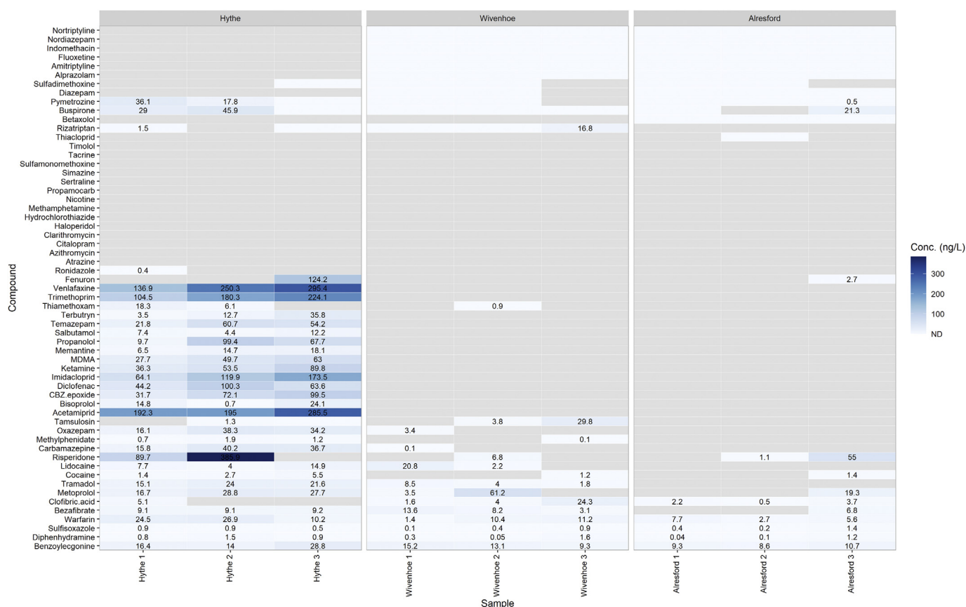
Fig. 4. Heatmap showing concentrations ( \text{ng L}^{-1} ) of CEC determined in surface water collected from each sampling site. Grey tiles indicate samples were below the limit of quantification.
