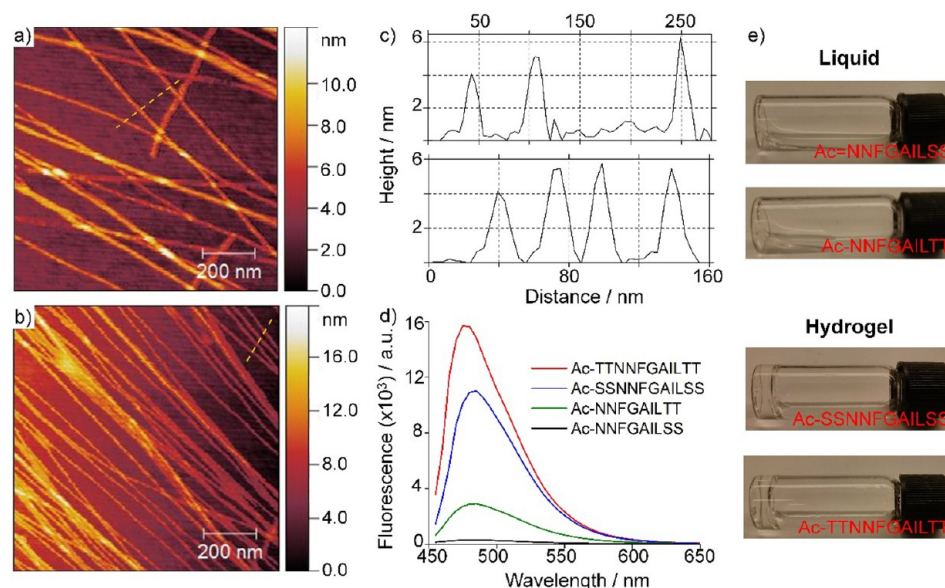
Figure 7. Effects of amino acid sequence on fibril morphologies, peptide aggregation, and hydrogelation behaviors. (a–c) AFM topographies of self-assembled nanoribbons: (a) Ac-SSNNFGAILSS and (b) Ac-TTNNFGAILTT. (c) Height profiles of the nanoribbons are shown along the dashed lines in the corresponding images (top: Ac-SSNNFGAILSS; bottom: Ac-TTNNFGAILTT). (d) ThT assay of the peptide solutions (2 mM), indicating the higher propensity of \beta -sheet formation for the extended peptides (ex. 440 nm and em. 485 nm). (e) Photos of the peptide solutions, in which hydrogelation was noted in the systems of extended peptide sequences (i.e., Ac-SSNNFGAILSS and Ac-TTNNFGAILTT). The peptide solutions (5 mM) were aged in phosphate buffer (20 mM, pH 7.5) for 2 days before gel inversion test.
