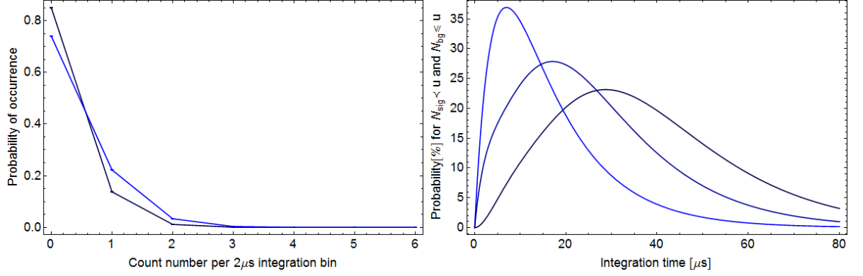
Figure 4.14: Using Poisson statistics to calculate the detection fidelity. LHS: The distribution of counts per 2\mu\text{s} integration time bin for the signal counts (lighter blue) and the background counts (darker blue). Fitting these distributions to a Poisson distribution gives estimates of the respective means as \bar{x}_{sig}^{fit} = 0.3008 \pm 0.0002 and \bar{x}_{bg}^{fit} = 0.1621 \pm 0.0003 . RHS: The joint probability for detecting a signal count level \geq u and a background count level < u as a function of integration time. Three values of u are shown; u = 3 is shown in the darkest blue; u = 2 is shown in the medium-toned blue; and u = 1 in the lightest blue. As u increases the peak fidelity decreases and occurs for larger \tau_{int} .
