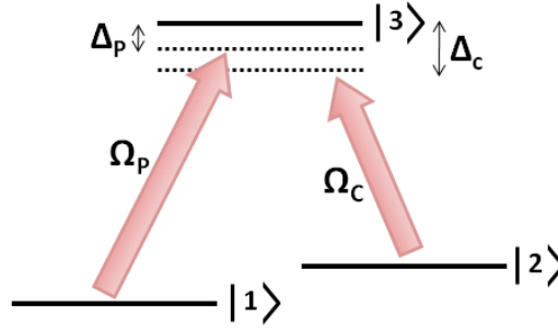
Figure 6.3: The three-level ‘lambda’ system, consisting of levels |1\rangle , |2\rangle and |3\rangle . The transitions are addressed by two coherent laser fields; \Omega_c and \Omega_p , with respective detunings \Delta_p = \omega_{31} - \omega_p and \Delta_c = \omega_{32} - \omega_c .
