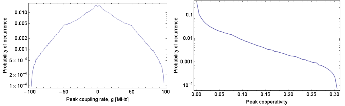
Figure 4.20: The probability of an atom having a given peak coupling rate, calculated by randomly assigning coordinates inside the cavity mode to one atom, one million times. The bounds for each coordinate are set by the cavity length and cavity waist. LHS: The probability of occurrence of a given peak coupling rate, g . The coupling rates are grouped into 1 MHz wide bins spanning a range -98 \rightarrow 98 MHz. RHS: The probability of occurrence of a given peak C . The peak cooperativities are grouped into 0.005 wide bins spanning a range 0 \rightarrow 0.31 .
