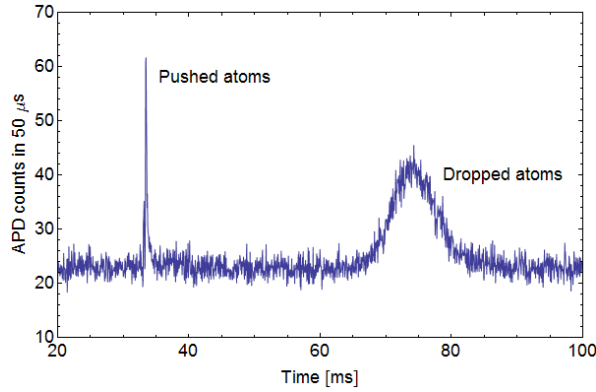
Figure 5.1: The counts measured at the APD averaged over ten shots of a push beam experiment. The reflection signal resulting from pushed atoms is clearly visible as the tall, narrow feature, centred at approximately 35 ms. The residual reflection signal from falling atoms is centred at approximately 75 ms. The relative signal heights are 2.70 \pm 0.09 for the pushed atoms and 1.75 \pm 0.02 for the dropped atoms (both in lab units), corresponding to collective cooperativities of 1.75 \pm 0.39 and 0.31 \pm 0.01 respectively. This implies that the pushed signal corresponds to N_{\text{eff}} = 5.5 atoms.
