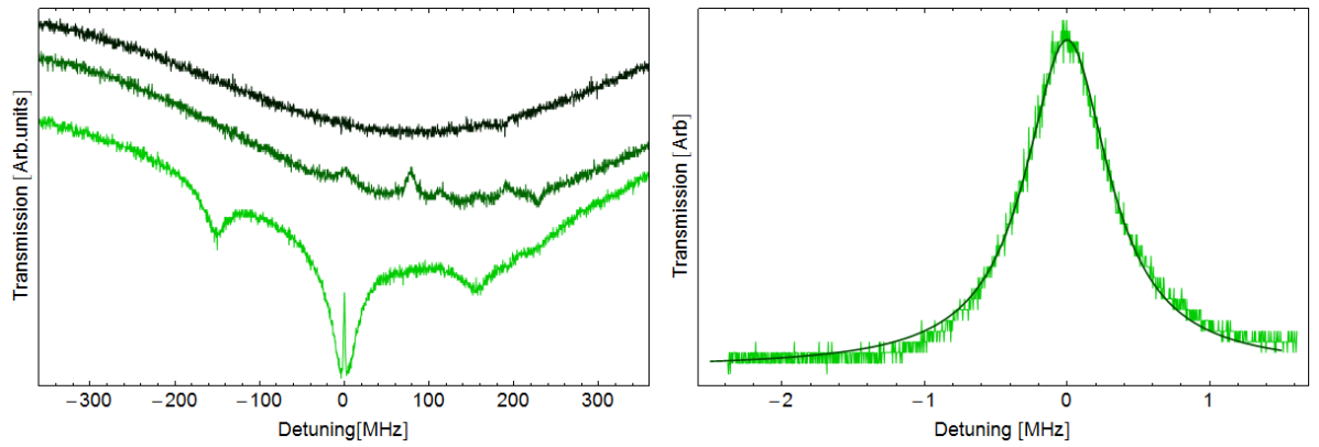
Figure 6.5: Electromagnetically induced transparency in an Rb vapour cell. LHS: The transmission profile of the probe beam is shown as \Delta_p is tuned across the ^{87}\text{Rb} |F=0\rangle \rightarrow |F=0, 1, 2\rangle manifold. The darkest green shows the Doppler-broadened absorption profile. The medium-toned green shows the saturated absorption spectrum of the same transitions, where now the probe beam is retro-reflected through the cell. The lightest green shows the same saturated absorption spectrum, but now with the co-propagating coupling laser present. The narrow EIT feature is clearly visible at zero detuning. RHS: A ‘zoomed in’ version of the EIT feature. Shown alongside the scan is the fitted Lorentzian lineshape, which estimates the HWHM to be 357 \pm 4 kHz.
