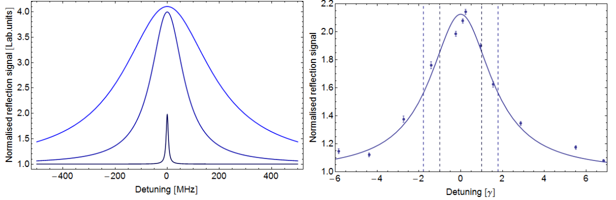
Figure 4.7: The reflection signal as a function of pump beam detuning. LHS: The reflection signal, calculated using Eq.(4.8), shown for three different coupling regimes. (g, \gamma) are kept constant at 2\pi \times (98, 3) MHz respectively, whilst the value of \kappa is changed. The dark blue shows \kappa = 2\pi \times 5200 MHz or \kappa \gg g , which is the regime we work in; the medium-toned blue shows \kappa = 2\pi \times 141 MHz, or \kappa = \sqrt{2g^2 - \gamma^2} and is the threshold for the strong coupling regime; the light blue shows \kappa = 2\pi \times 50 MHz or \kappa < g , well into the strong coupling regime. The increased height and width of the lineshape as \kappa reduces (and thus C_N increases) is visible. RHS: The normalised reflection signal measured as a function of pump beam detuning (shown in units of \gamma ). A fit to Eq.(4.8) is shown alongside the data, which estimates C_N = 0.39 \pm 0.01 . The inner pair of dashed lines indicate the bare-atom linewidth of \gamma . The outer pair of dashed lines indicate the Purcell-enhanced linewidth of 2C_N\gamma .
