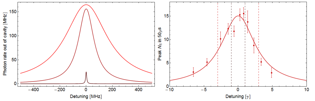
Figure 4.8: The fluorescence signal as a function of pump beam detuning. LHS: The calculated fluorescence signal plotted for three coupling regimes, using Eq.(4.9). (g, \gamma, \Omega) are kept constant at 2\pi \times (98, 3, 10) MHz respectively, whilst the value of \kappa is changed. The dark red shows \kappa = 5200 MHz or \kappa \gg g , which is the regime we work in; the medium-toned red shows \kappa = 141 MHz, or \kappa = \sqrt{2g^2 - \gamma^2} and is the threshold for the strong coupling regime; the light red shows \kappa = 50 MHz or \kappa < g , well into the strong coupling regime. The increased height and width of the lineshape as \kappa reduces (and thus C_N increases) is visible. RHS: The average peak fluorescence counts, N_{fl} , collected at the APD in a 50 \mu s time bin versus detuning, \Delta_a of the pumping beam. The fit shown is to Eq.(4.9), which estimates C_N = 1.01 \pm 0.16 .
