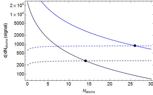
Figure 4.15: The range of N_{\text{eff}} which can be discriminated by our atom detector. The solid lines show the differentiated signal with respect to N_{\text{eff}} as a function of N_{\text{eff}} , for two different pumping rates: 810 kCounts/sec (in lighter blue) and 81 kCounts/sec (in darker blue). The dashed lines show the signal fluctuations as a function of N_{\text{eff}} . Where the solid and dashed line of each colour meet, shown by the solid points, indicates the upper limit of the detection range. For the higher pumping rate this occurs at N_{\text{eff}} = 26.2 and for the lower pumping rate this occurs at N_{\text{eff}} = 14.1 .
