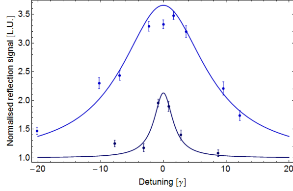
Figure 5.5: The normalised reflection signal with cavity pump beam detuning. The lighter blue dataset corresponds to a detuning scan across the first pulse in a multi-push experiment and the darker blue dataset corresponds to the same scan for the seventeenth pulse. Lorentzian fits to each dataset are shown alongside, producing estimates of C_N = 3.55 \pm 0.11 and C_N = 0.40 \pm 0.04 , respectively.
