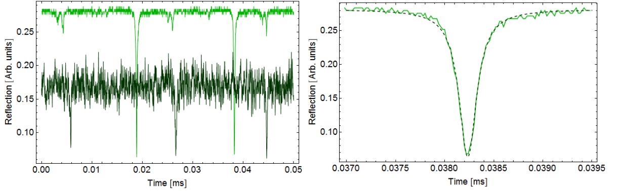
Figure 3.3: The reflected cavity fringes. LHS: The reflected cavity fringes for the 804 nm light used for locking and trapping (shown in light green) and the 780 nm light used for atom detection (shown in dark green), taken whilst the cavity length is being scanned. The relative amplitudes should not to be directly compared; the 780 nm is measured using a low pass filter to convert APD counts into an analogue voltage for the purposes of locking whilst the 804 nm is measured using a photodiode. RHS: A ‘zoomed’ scan of just one cavity fringe. The dashed line indicates an inverted Lorentzian lineshape, which is a good approximation for the cavity fringes.
