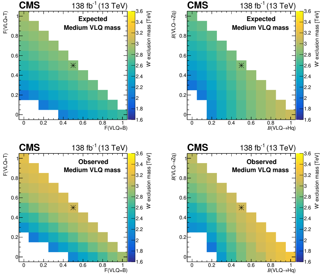
Figure 8. Expected (upper) and observed (lower) 95% CL limits for generalized hypotheses varying the fraction of tB ( F(VLQ=B) ) and bT ( F(VLQ=T) ) from the W' decay (left), and the VLQ branching fraction to qH and qZ (right). The asterisk marker signifies the branching fractions for the benchmark model.
