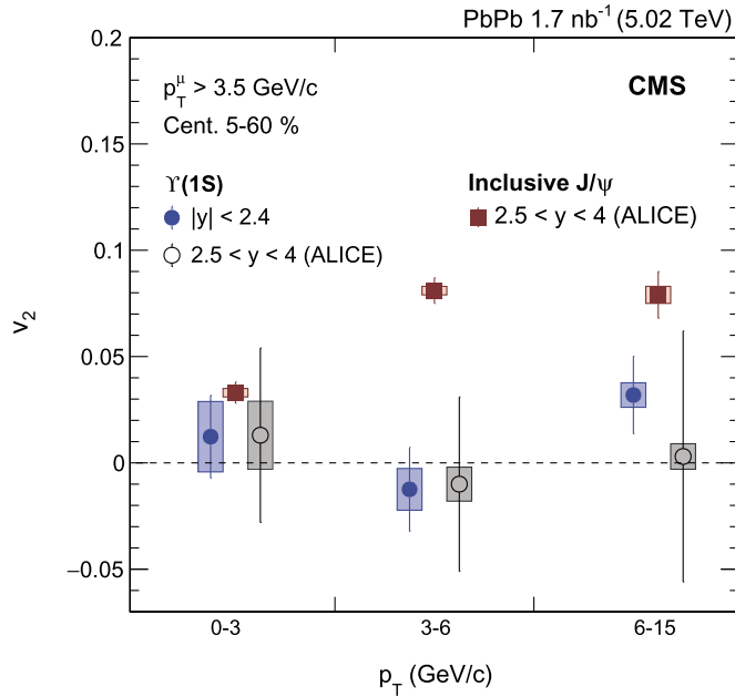
Fig. 4. The v_2 for Y(1S) mesons as a function of p_T in the rapidity range |y| < 2.4 compared with the ALICE results for Y(1S) (open circles) and J/ψ (full squares) mesons measured in 2.5 < y < 4 [24]. All results are obtained in the range 0 < p_T < 15 GeV/c and centrality interval 5–60%. The vertical bars denote statistical uncertainties, and the rectangular boxes show the total systematic uncertainties.
