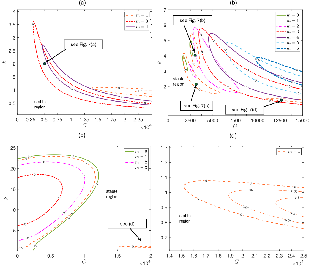
FIG. 6. Neutral curves for m \geq 0 , when \mu = 0.5 , R_2 = 1.3 , R_0 = 0.1 , J = 100 , W = 0 , I = 1 , Z = 0 . In panel (a) B = 100 , \chi_1 = 5 , \chi_2 = 0 , (b) B = 500 , \chi_1 = 5 , \chi_2 = 0 , and in panel (c) B = 100 , \chi_1 = 0 , \chi_2 = 5 . (d) Region 3 enlarged. As B increases, it extends to the left when \chi_1 > \chi_2 , but modes are stabilized when \chi_2 > \chi_1 .
