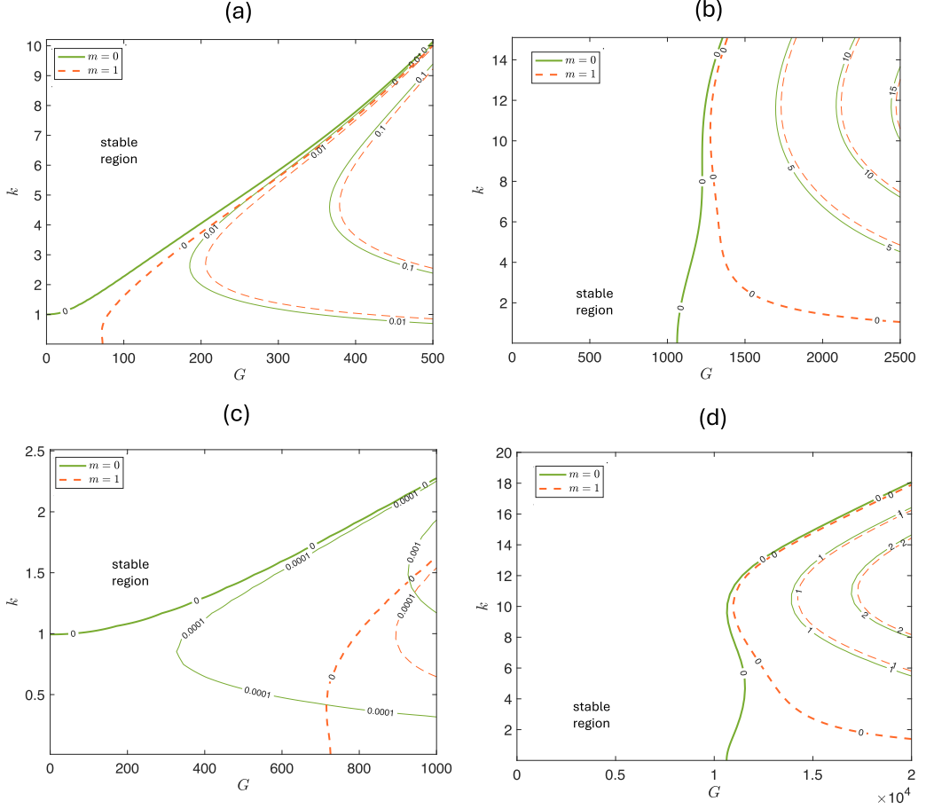
FIG. 11. Growth rates when \mu = 0.5 , R_2 = 1.3 , R_0 = 0.9 , \chi_1 = 5 , \chi_2 = 0 , I = 1 , Z = 0 for (a) J = 1 , B = 0 (FBBM), (b) J = 1 , B = 100 , (c) J = 100 , B = 0 (FBBM), and (d) J = 100 , B = 100 . Increasing B shifts the unstable region to the right.
