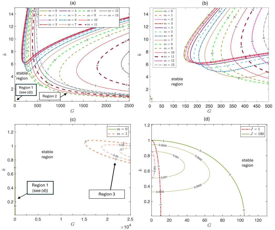
FIG. 2. Growth rates when \mu = 0.5 , R_2 = 1.3 , R_0 = 0.1 , W = 0 , B = 0 . (a) Neutral curves when J = 1 . Two regions of instability exist; region 1 consists of m = 0 unstable capillary modes for G \leq G_L and region 2 consists of m \geq 0 interfacial modes for G \geq G_R . (b) Close-up of panel (a). (c) J = 100 and two regions of instability exist, regions 1 and 3. Increasing J has shifted region 2 to the right, so that region 2 exists past region 3, and G_R is at the onset of region 3. (d) Region 1 m = 0 unstable modes when J = 1 and J = 100 , where G_L increases as J increases and only m = 0 modes are unstable. (Figure adapted from Fig. 3 in FBBM.)
