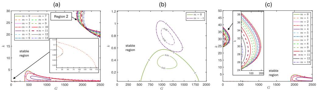
FIG. 15. Growth rates when \mu = 1.5 , R_2 = 2 , R_0 = 0.9 , J = 1 , \chi_1 = 5 , \chi_2 = 0 , where in panel (a) W = 100 , B = 0 and in panel (b) W = 100 , B = 100 , I = 1 , Z = 1 . In panel (c) W = 500 , B = 0 . Panels (a) and (c) are adapted from FBBM.
