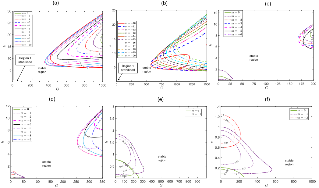
FIG. 5. Growth rates when \mu = 0.5 , R_2 = 1.3 , R_0 = 0.1 , W = 0 , I = 1 , where J = 1 in panels (a)–(d), and J = 100 in panels (e), (f). In panels (a), (b) B = 10 , \chi_1 = 5 , \chi_2 = 0 , with (a) Z = 1 , (b) Z = 2 . In panels (c), (d) B = 1 , \chi_1 = 0 , \chi_2 = 5 , with (c) Z = 1 , (d) Z = 2 . In panels (e), (f) B = 1 , \chi_1 = 0 , \chi_2 = 5 , with (e) Z = 1 , (f) Z = 2 . m < 0 modes can be the most unstable. If \chi_1 > \chi_2 , then region 1 is stabilized and region 2 is pushed to the right as B or Z increases. If \chi_2 > \chi_1 , then increasing Z increases G_L , but region 2 is shifted further to the right, increasing G_R .
