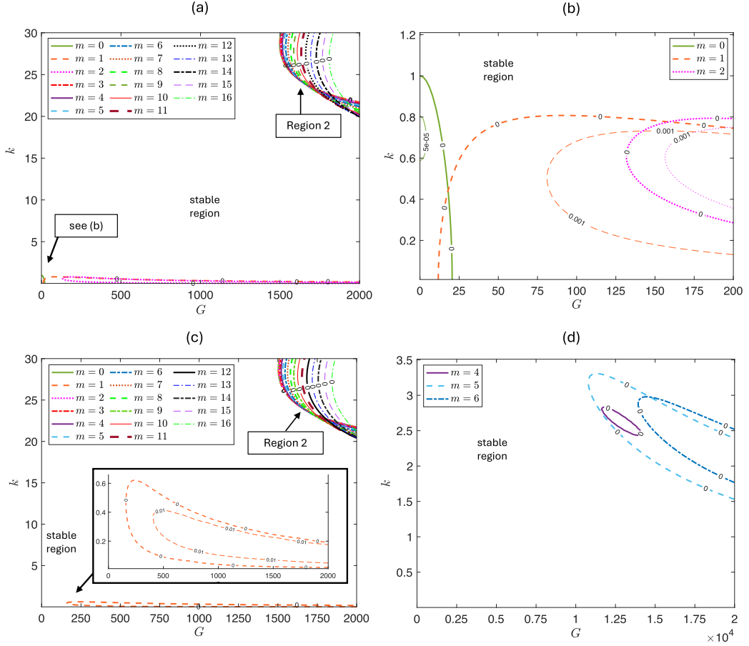
FIG. 12. Growth rates when \mu = 1.5 , R_2 = 2 , R_0 = 0.9 , W = 0 , \chi_1 = 5 , \chi_2 = 0 , I = 1 , Z = 0 , and in panel (a) J = 1 , B = 0 , where panel (b) shows an enlarged image of the lower region (FBBM), in panel (c) J = 1 , B = 1 , (d) J = 100 , B = 300 . An azimuthal field has a stabilizing effect, but past a critical strength unstable magnetic modes appear.
