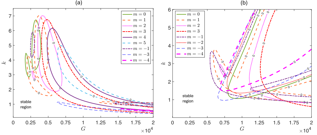
FIG. 9. Neutral curves when \mu = 0.5 , R_2 = 1.3 , R_0 = 0.1 , J = 100 , W = 0 , B = 100 , \chi_1 = 5 , \chi_2 = 0 , I = 1 . In panel (a) Z = 1 , (b) Z = 5 . Increasing the axial field strength, increases the range of stable G , pushing the magnetic region to the right.
