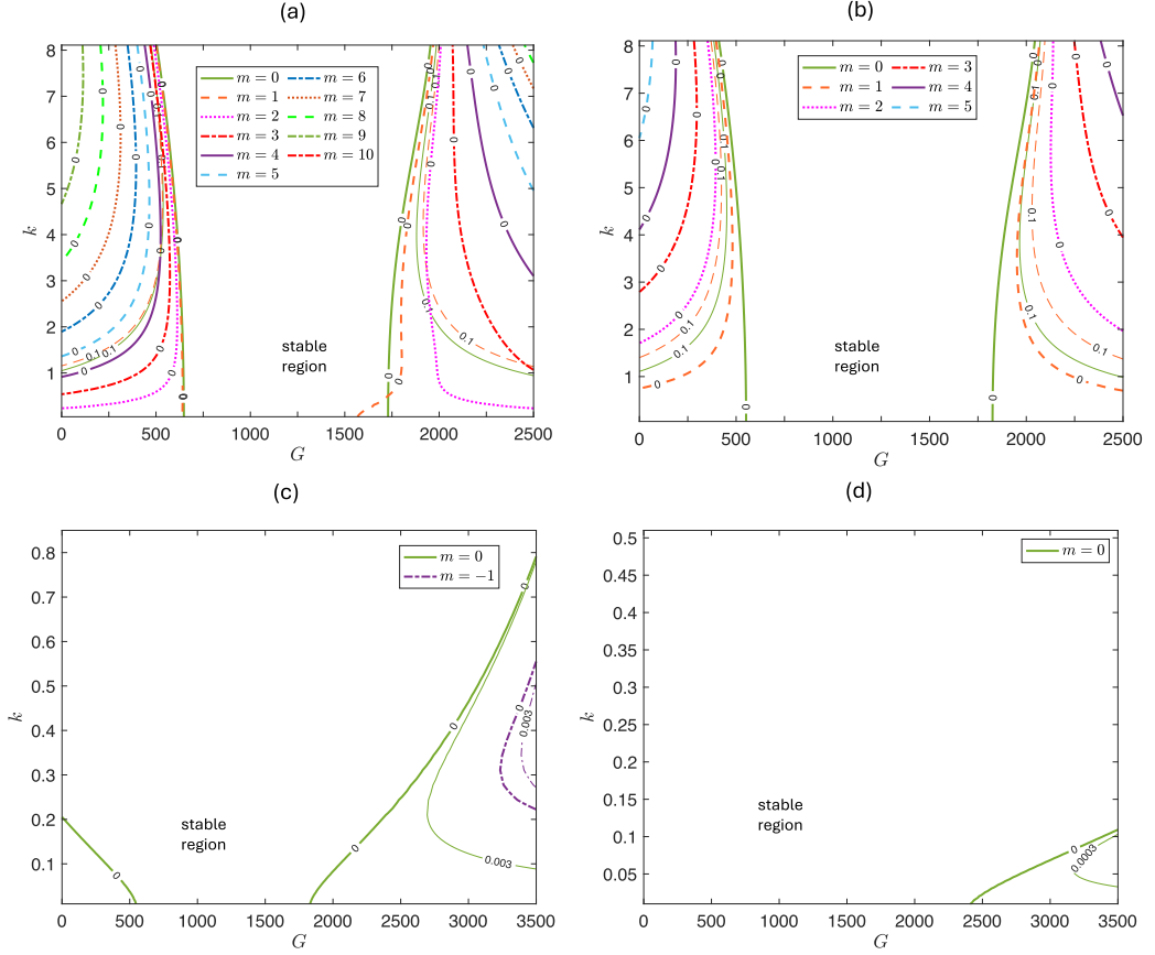
FIG. 14. Growth rates when \mu = 0.5 , R_2 = 1.3 , R_0 = 0.9 , J = 1 , W = 50 , \chi_1 = 5 , \chi_2 = 0 , and in panel (a) B = 0 (FBBM), (b) B = 10 , I = 1 , Z = 0 , (c) B = 10 , I = 1 , Z = 5 , and (d) B = 100 , I = 1 , Z = 5 .
