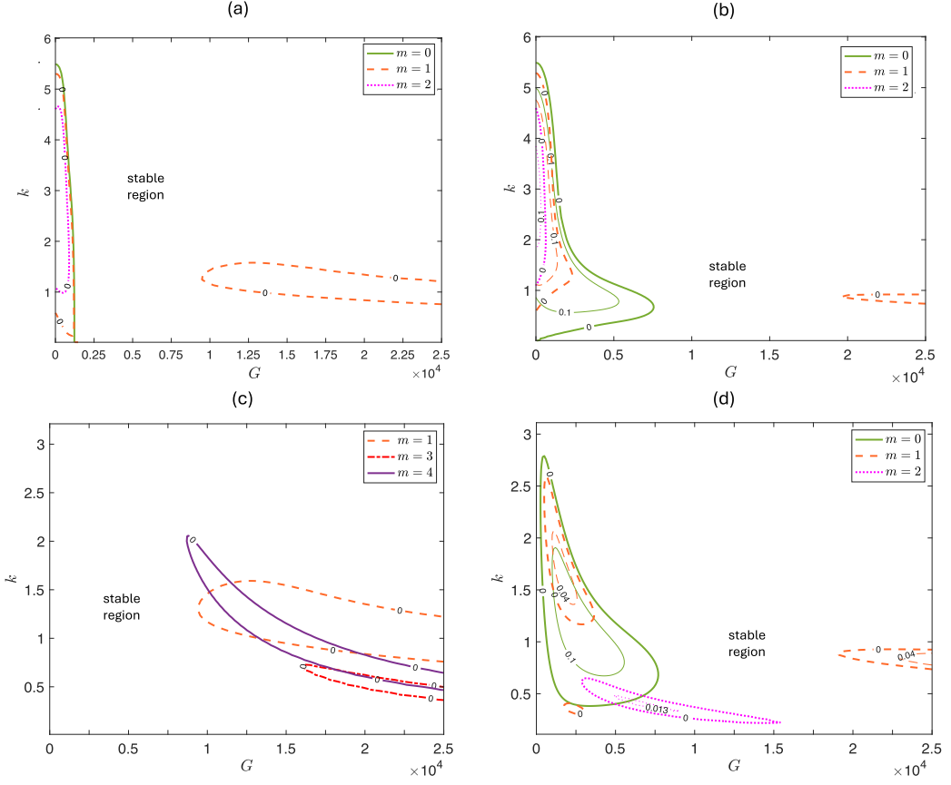
FIG. 13. Growth rates when \mu = 0.5 , R_2 = 1.3 , R_0 = 0.1 , \chi_1 = 5 , \chi_2 = 0 , I = 1 , Z = 0 , and in panel (a) W = -1000 , B = 0 (FBBM), (b) W = 1000 , B = 0 (FBBM), (c) W = -1000 , B = 100 , (d) W = 1000 , B = 40 . An azimuthal field stabilizes instabilities caused by the moving rod at low G , but unstable magnetic modes can be triggered.
