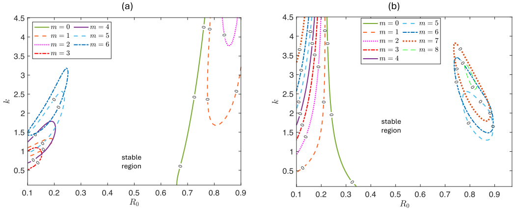
FIG. 10. Neutral curves for m \geq 0 , when G = 20000 , J = 100 , W = 0 , B = 200 , \chi_1 = 5 , \chi_2 = 0 , I = 1 , Z = 0 . In panel (a) \mu = 0.5 , R_2 = 1.3 , and in panel (b) \mu = 1.5 , R_2 = 2.0 .
