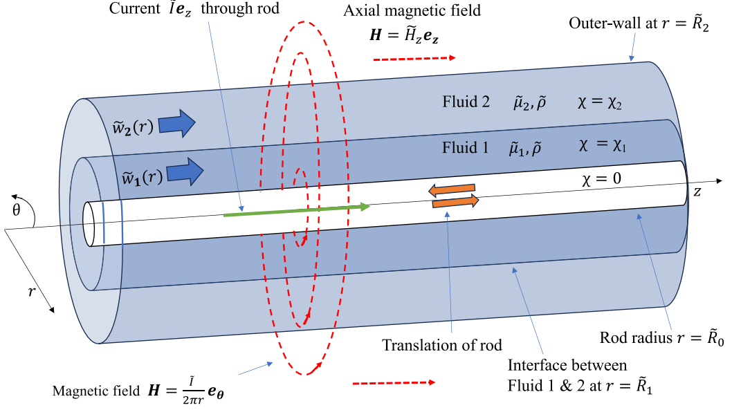
FIG. 1. Schematic of the base state.
