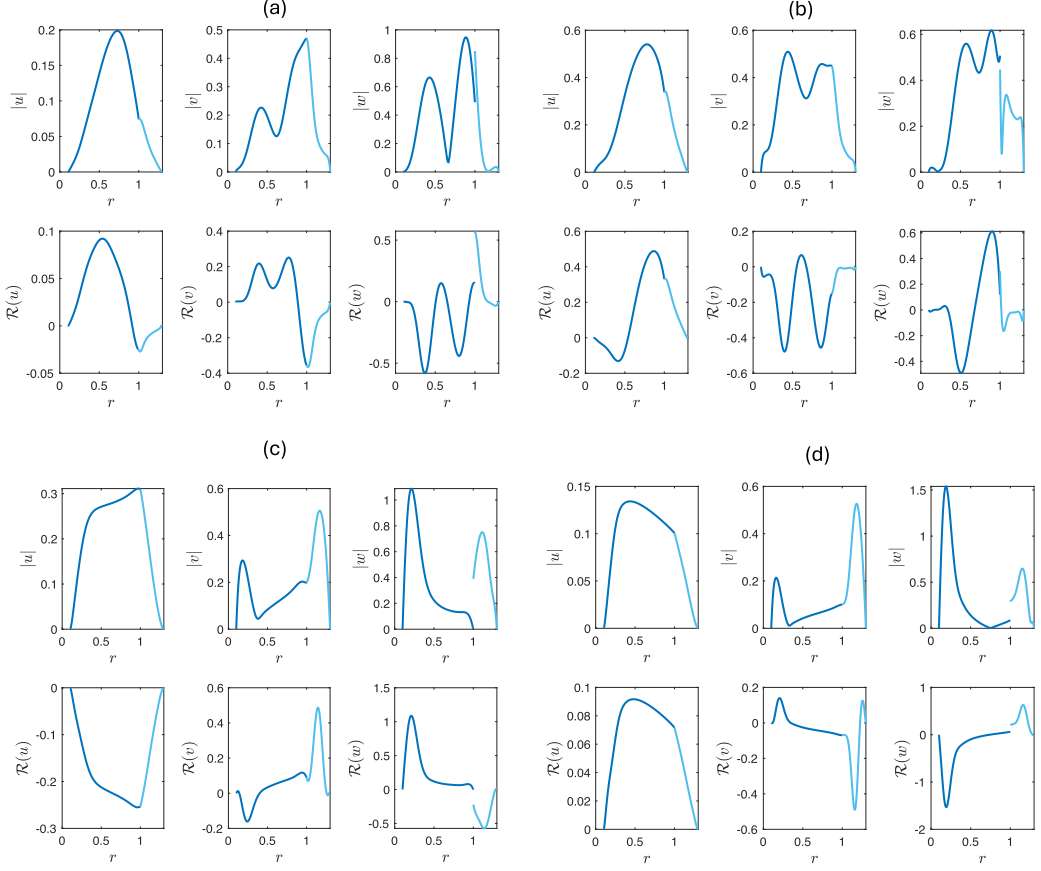
FIG. 7. Eigenfunctions when \mu = 0.5 , R_2 = 1.3 , R_0 = 0.1 , J = 100 , W = 0 , \chi_1 = 5 , \chi_2 = 0 , I = 1 , Z = 0 . In panel (a) B = 100 , m = 3 , k = 2 , G = 5000 when s = 0.06088 - 25.88i . In panels (b)–(d) B = 300 , m = 1 , where in panel (b) k = 4 , G = 3000 , s = 0.042 - 31.695i , (c) k = 2 , G = 3000 , s = 0.036 - 7.958i , and (d) k = 1.1 , G = 12\,500 , s = 0.011 - 14.223i .
