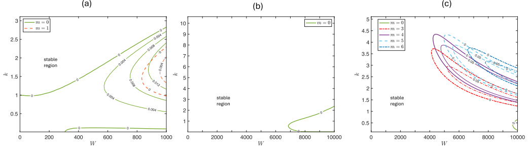
FIG. 16. Growth rates when G = 0 , \mu = 0.5 , R_2 = 1.3 , R_0 = 0.1 , J = 100 , \chi_1 = 5 , \chi_2 = 0 , I = 1 , Z = 0 and in panel (a) B = 0 , (b) B = 100 , and (c) B = 200 .
