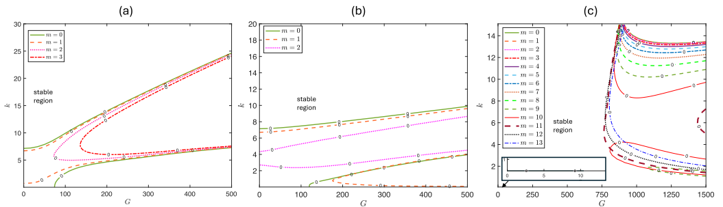
FIG. 4. Neutral curves when the outer fluid is more magnetic and \mu = 0.5 , R_0 = 0.1 , J = 1 , W = 0 , B = 10 , \chi_1 = 0 , \chi_2 = 5 . In panel (a) R_2 = 1.3 , I = 1 , Z = 0 , (b) R_2 = 2 , I = 1 , Z = 0 , (c) R_2 = 1.3 , I = 0 , Z = 1 . When the outer fluid is more magnetic, an axial field shifts region 2 to the right, and an azimuthal field destabilizes modes so that regions 1 and 2 merge.
