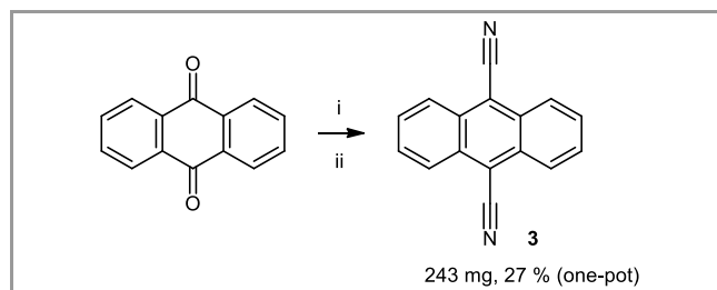
Scheme 2 One-pot synthesis of 9,10-dicyanoanthracene 3 from 9,10-anthraquinone: nucleophilic attack (i): TMS-CN, CsF, acetonitrile, 0°C, 5 h; reductive aromatization (ii): \text{PCl}_3 , DMF, acetonitrile, 0°C-rt, overnight.
