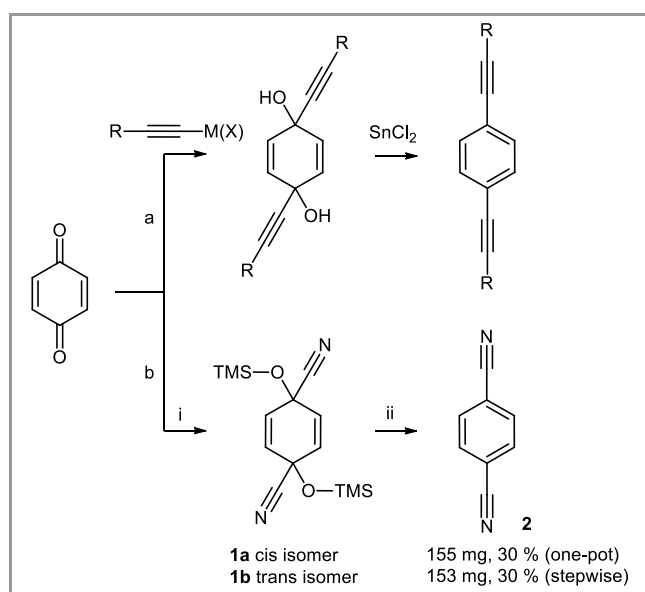
Scheme 1 (a) Well-established synthesis of ethynyl substituted aromatic compounds. (b) Novel synthesis of cyanated aromatic compounds: nucleophilic attack (i): TMS-CN, CsF, acetonitrile, 0°C, 10 min; reductive aromatization (ii): \text{PCl}_3 , DMF, acetonitrile, 0°C-rt, 1.5 h.
