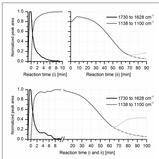
Figure 1 In-situ IR spectroscopic measurements of the reactions toward 1a-b (i) and 2 (ii): stepwise (top) and one-pot reaction (bottom); peaks integrated from 1730 to 1628 \text{cm}^{-1} (carbonyl vibrational bands), 1138 to 1100 \text{cm}^{-1} (intermediate peak); solid lines: measured values, dotted lines: expected values (deviation attributed to precipitation at the IR probe).
