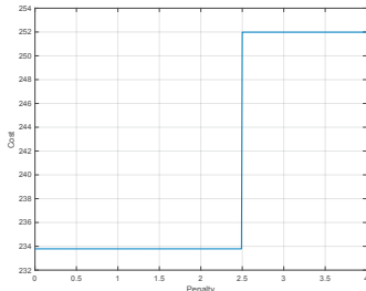
Fig. 8. Trend of agent 3's costs (in euro cents) as his declaration varies.
